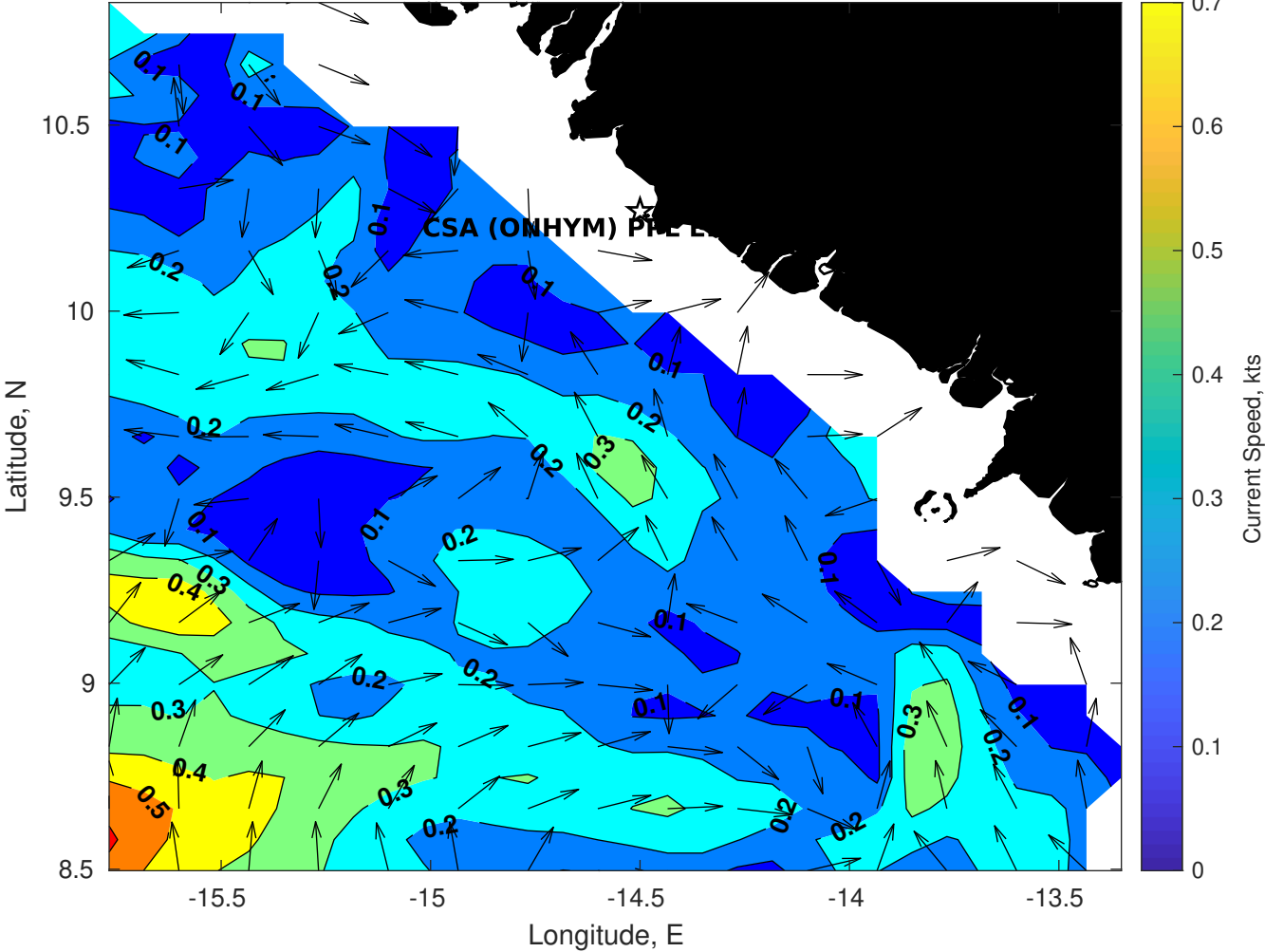
Surface Currents for CSA (ONHYM) PPL EBS - Guinea at 22-Oct-2025 00:00:00
