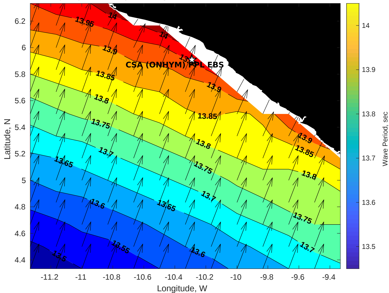
Wave Period (sec) for CSA (ONHYM) PPL EBS - Liberia at 22-Oct-2025 21:00:00
