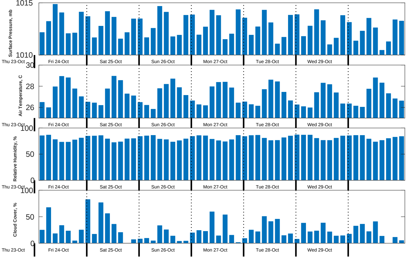
Met Forecast for CSA (ONHYM) PPL EBS - Liberia from 24-Oct-2025 00:00:00 to 31-Oct-2025 00:00:00
