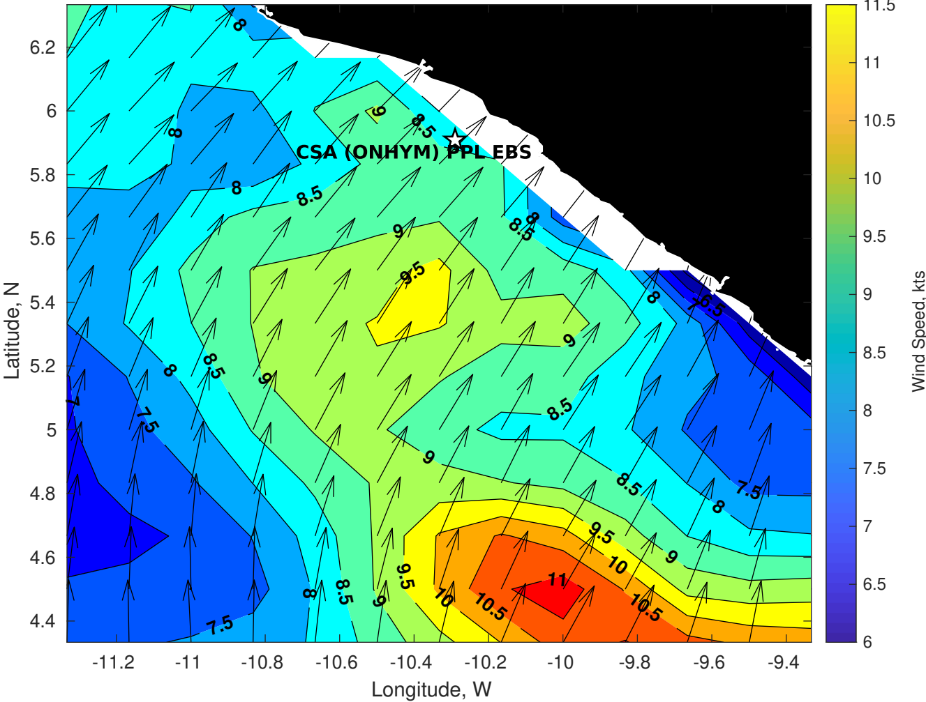
Winds (kts) for CSA (ONHYM) PPL EBS - Liberia at 22-Oct-2025 21:00:00
