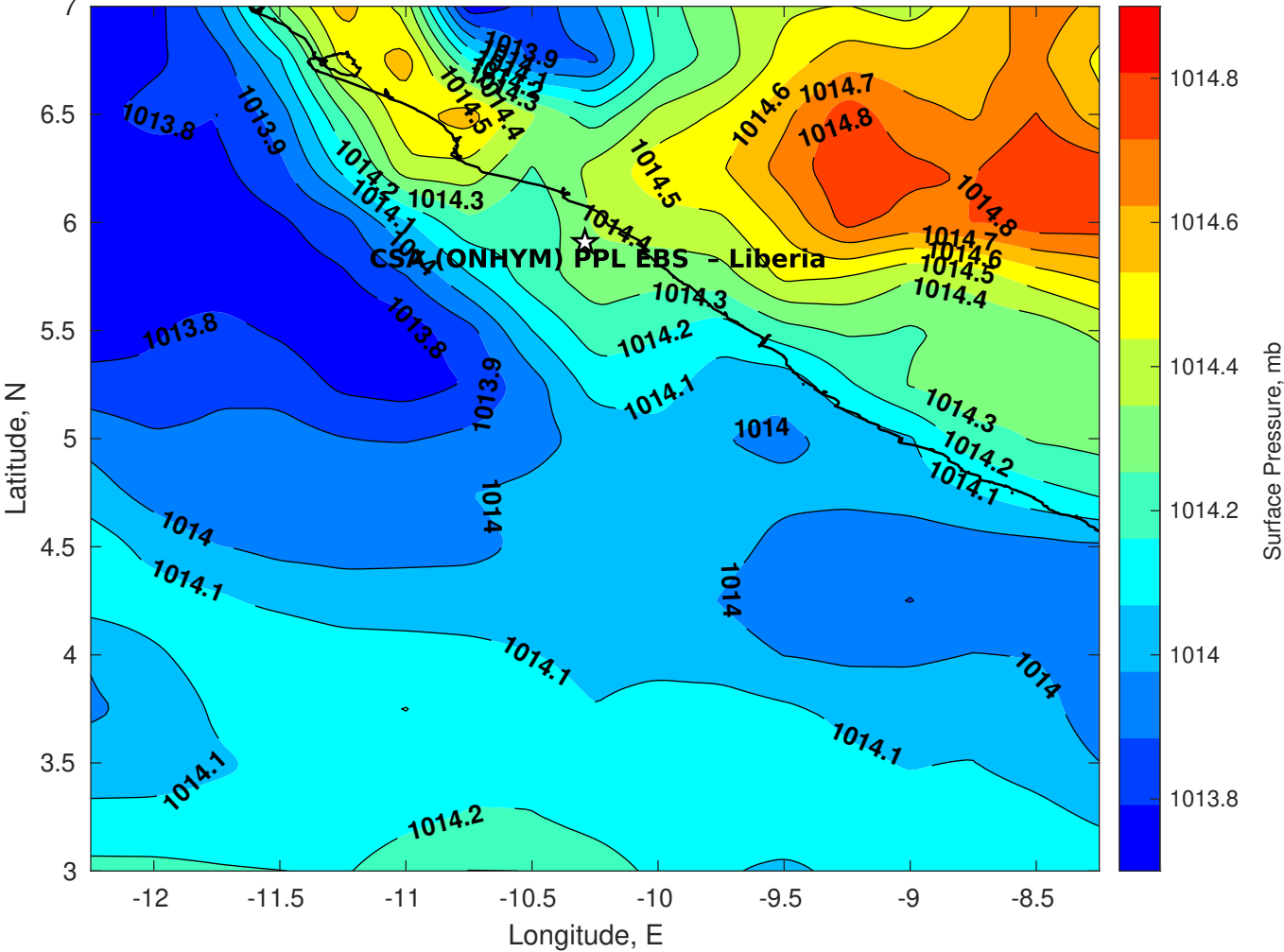
Surface Pressure (mb) for CSA (ONHYM) PPL EBS - Liberia at 24-Oct-2025 00:00:00
