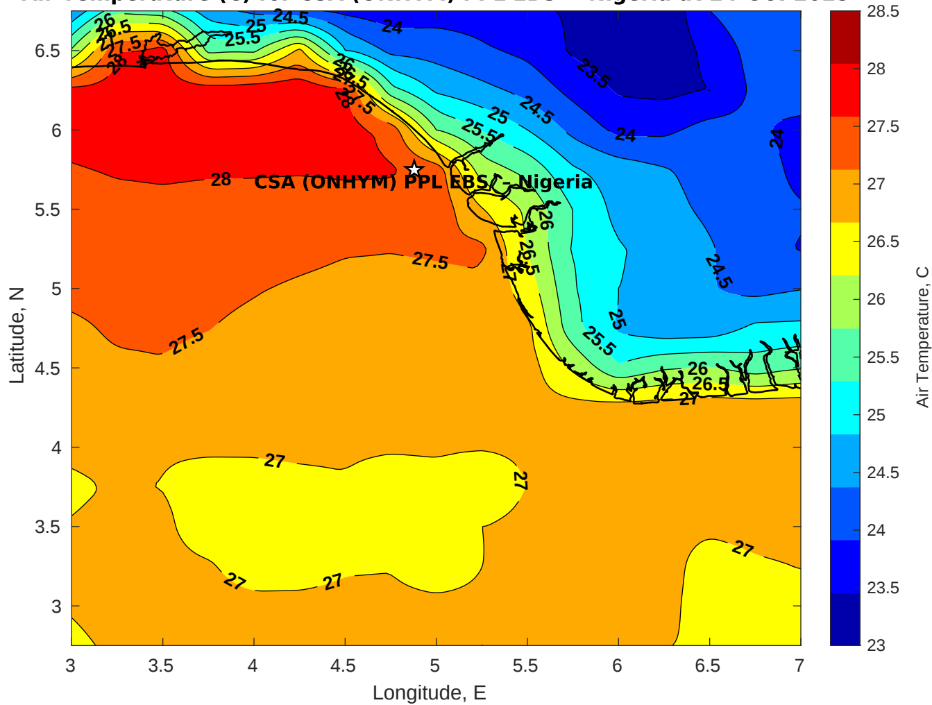
Air Temperature (C) for CSA (ONHYM) PPL EBS - Nigeria at 24-Oct-2025
