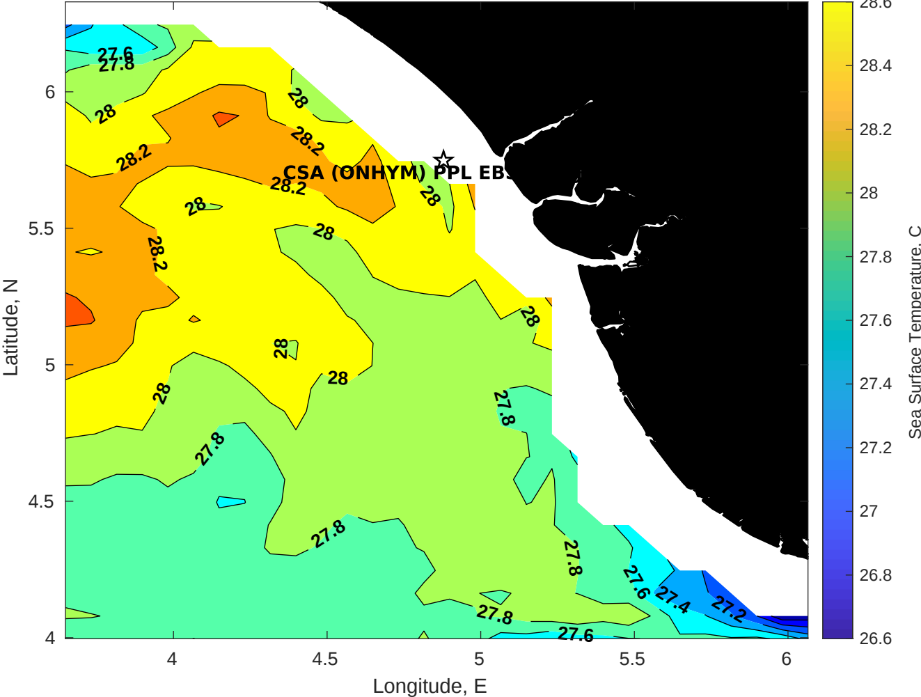
SST for CSA (ONHYM) PPL EBS - Nigeria at 22-Oct-2025 00:00:00
