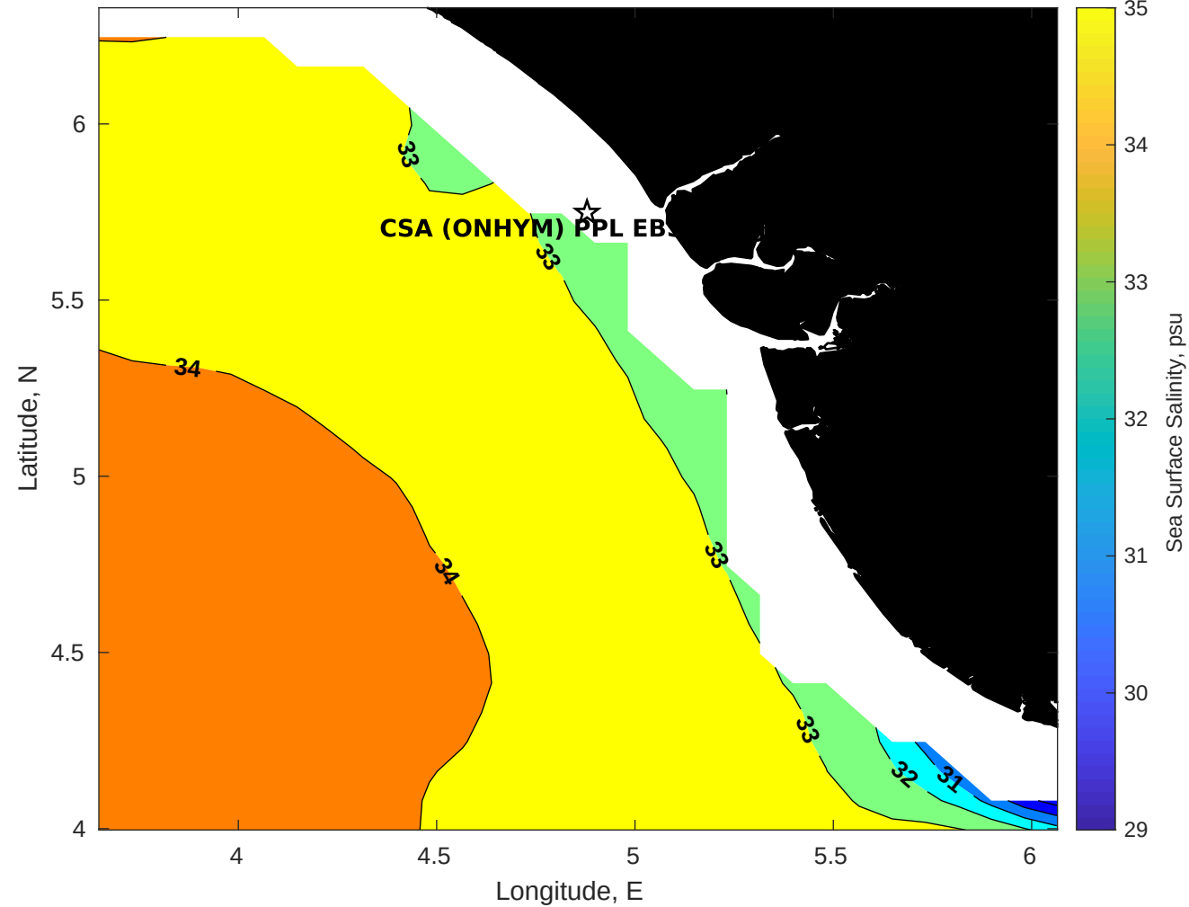
Surface Salinity for CSA (ONHYM) PPL EBS - Nigeria at 22-Oct-2025 00:00:00
