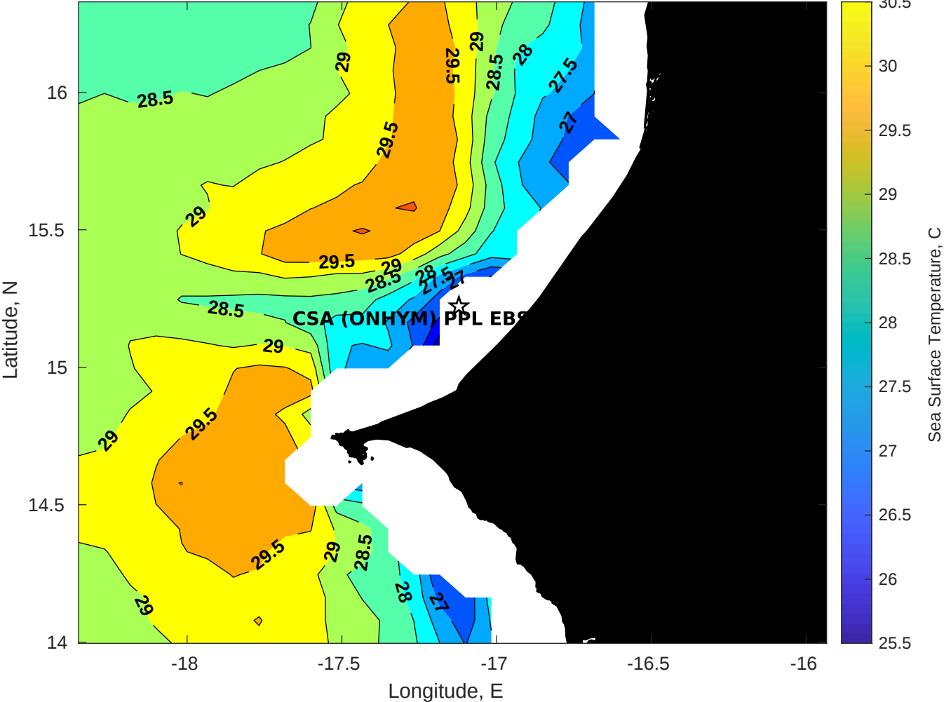
SST for CSA (ONHYM) PPL EBS - Senegal at 22-Oct-2025 00:00:00
