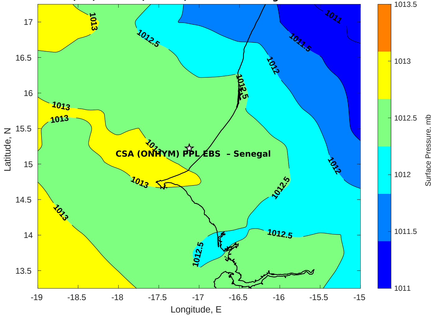
Surface Pressure (mb) for CSA (ONHYM) PPL EBS - Senegal at 25-Oct-2025 00:00:00
