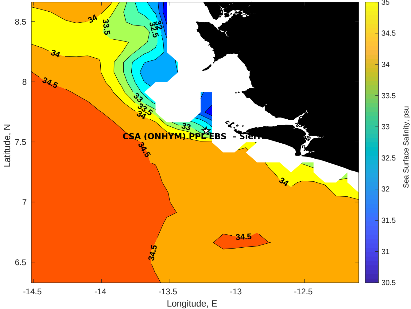
Surface Salinity for CSA (ONHYM) PPL EBS - Sierra Leone at 22-Oct-2025 00:00:00
