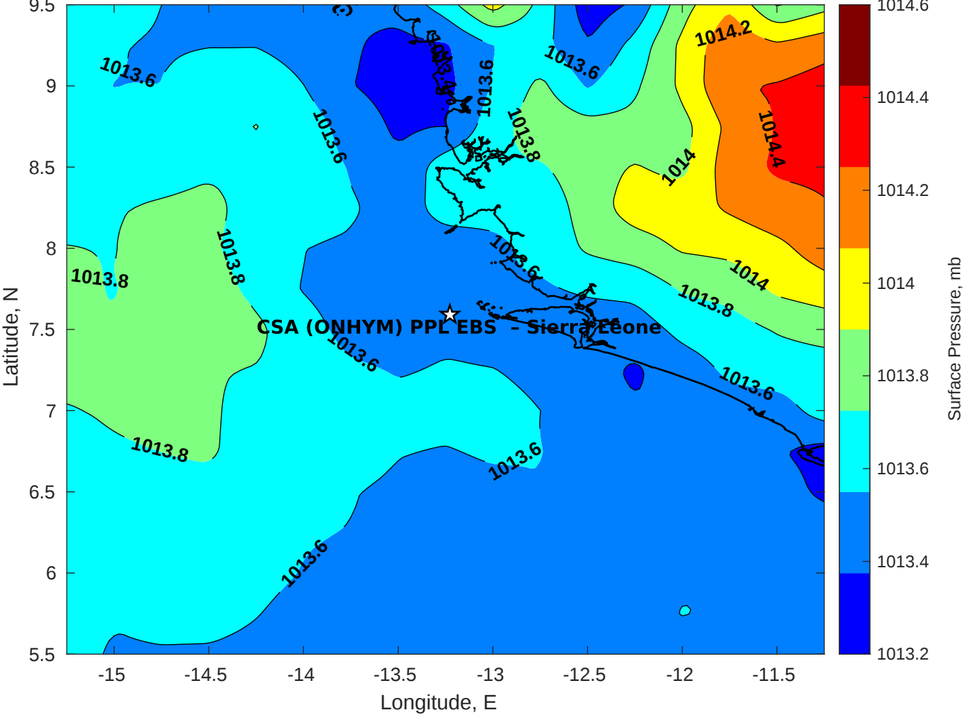
Surface Pressure (mb) for CSA (ONHYM) PPL EBS - Sierra Leone at 26-Oct-2025 00:00:00
