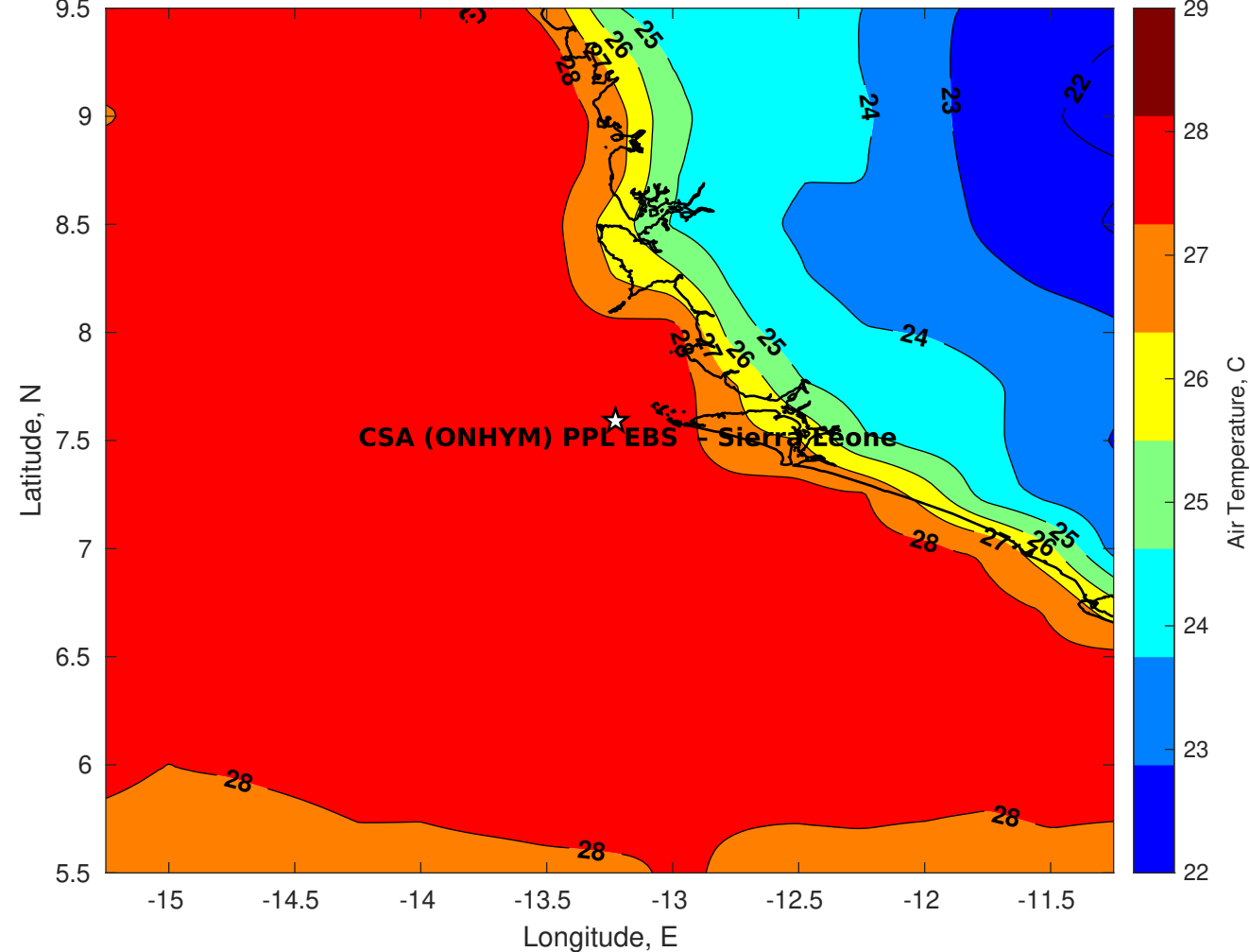
Air Temperature (C) for CSA (ONHYM) PPL EBS - Sierra Leone at 24-Oct-2025
