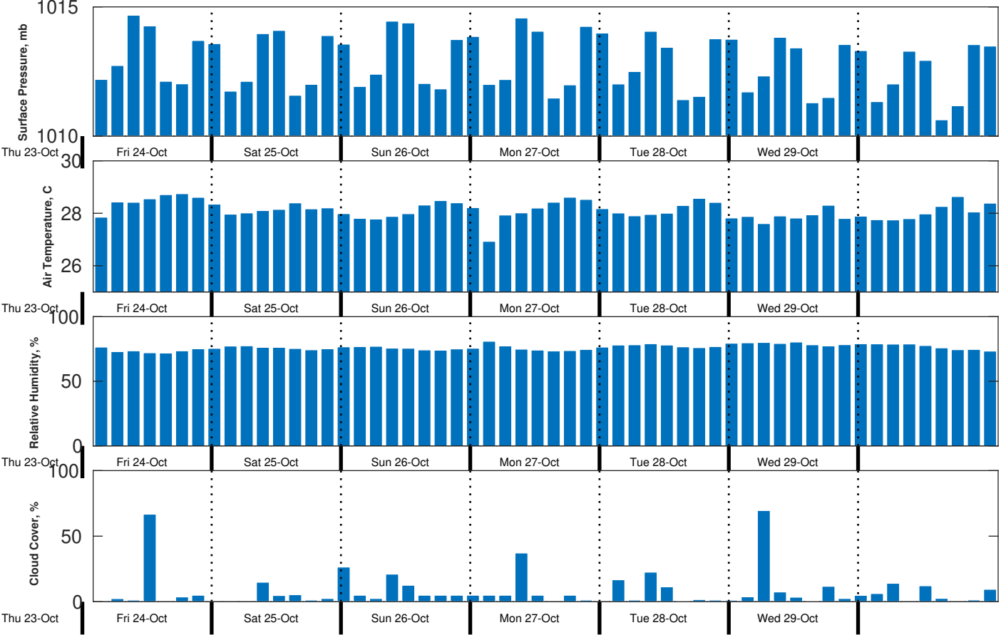
Met Forecast for CSA (ONHYM) PPL EBS - Sierra Leone from 24-Oct-2025 00:00:00 to 31-Oct-2025 00:00:00
