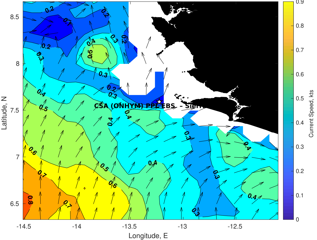
Surface Currents for CSA (ONHYM) PPL EBS - Sierra Leone at 22-Oct-2025 00:00:00
