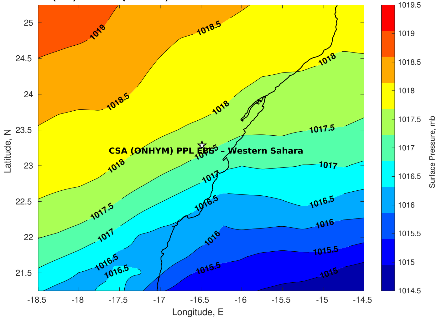
Surface Pressure (mb) for CSA (ONHYM) PPL EBS - Western Sahara at 24-Oct-2025 00:00:00
