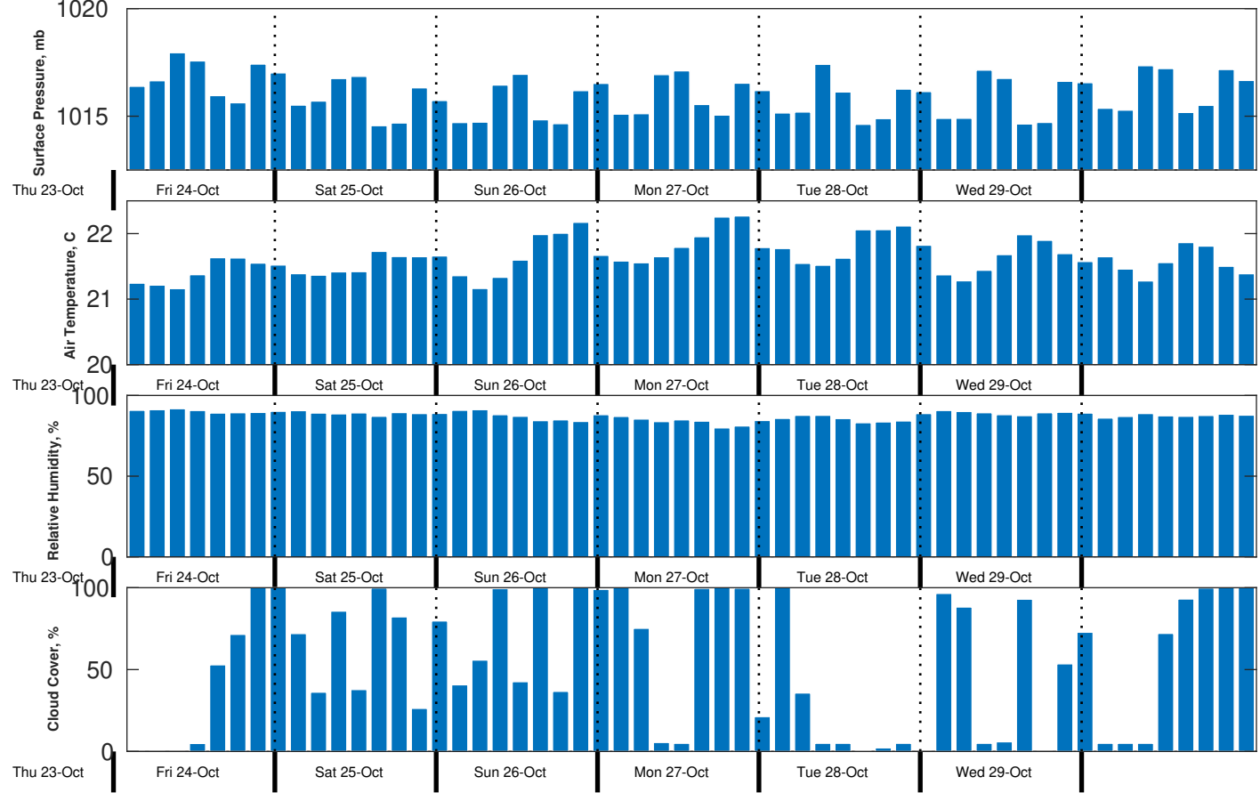
Met Forecast for CSA (ONHYM) PPL EBS - Western Sahara from 24-Oct-2025 00:00:00 to 31-Oct-2025 00:00:00
