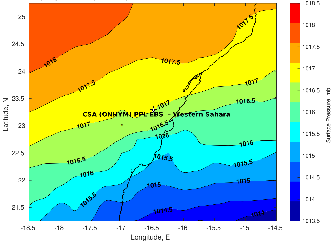
Surface Pressure (mb) for CSA (ONHYM) PPL EBS - Western Sahara at 25-Oct-2025 00:00:00
