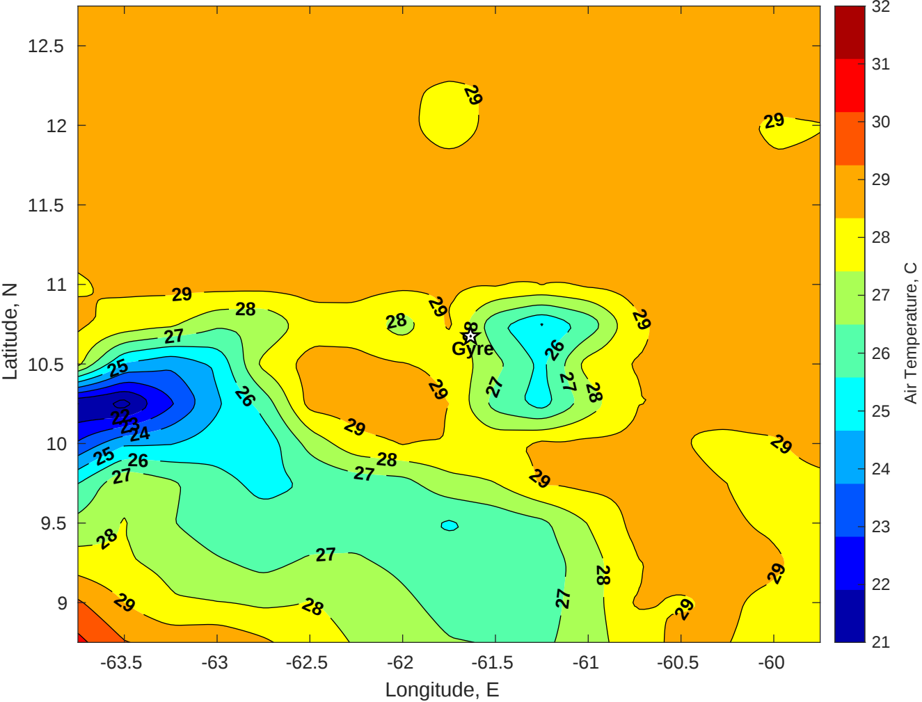
Air Temperature (C) for Gyre at 24-Oct-2025
