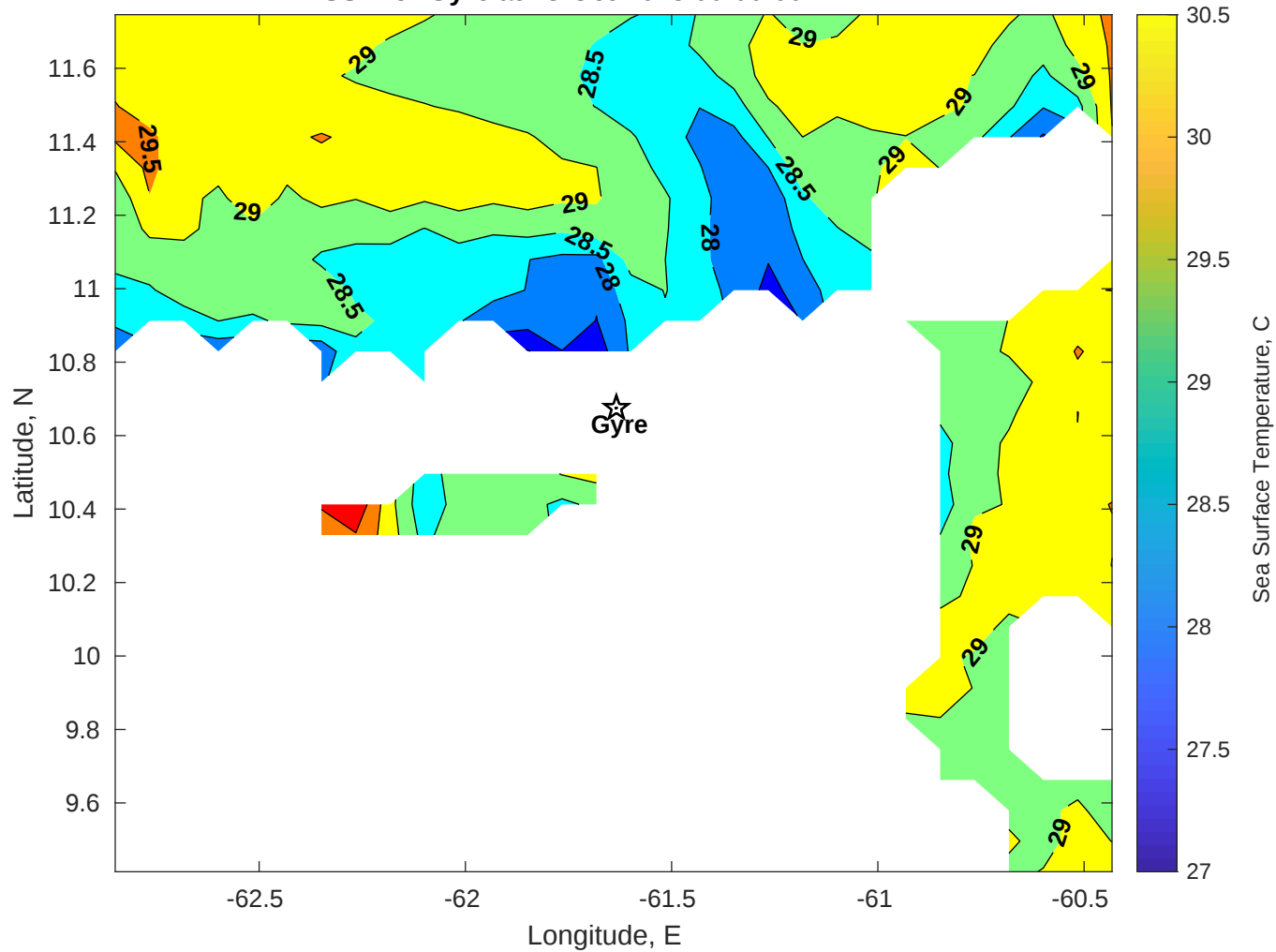
SST for Gyre at 23-Oct-2025 00:00:00
