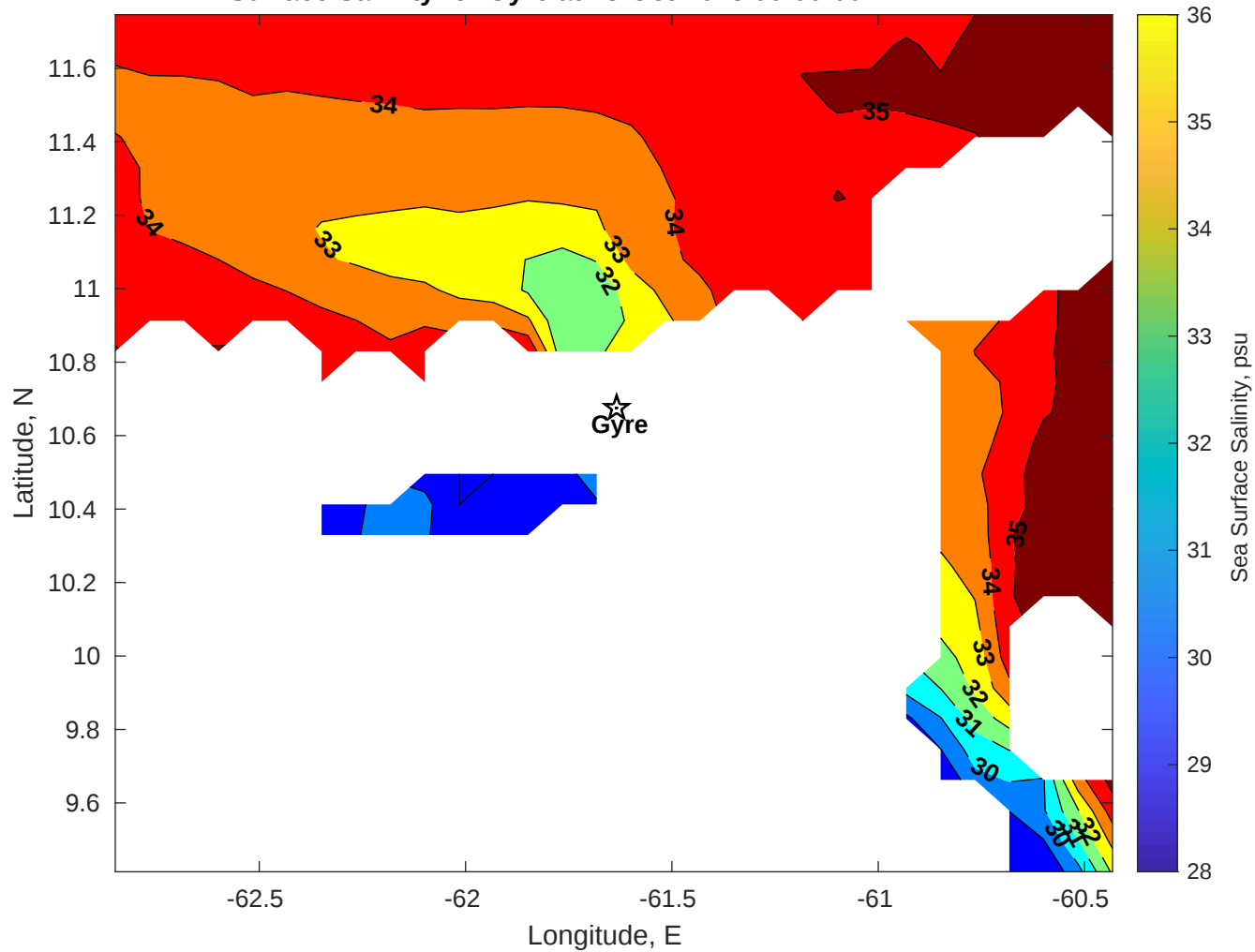
Surface Salinity for Gyre at 23-Oct-2025 00:00:00
