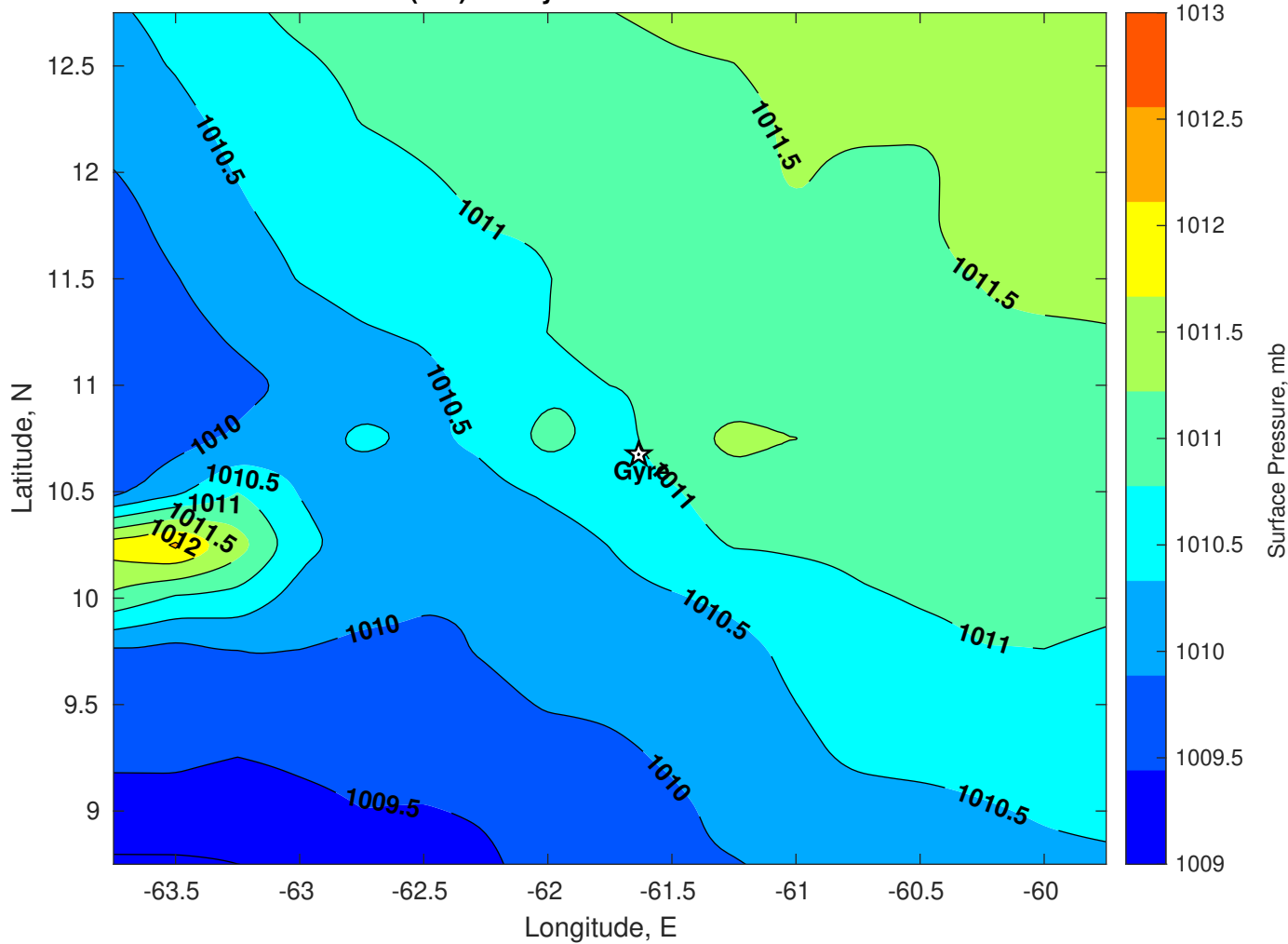
Surface Pressure (mb) for Gyre at 26-Oct-2025 00:00:00
