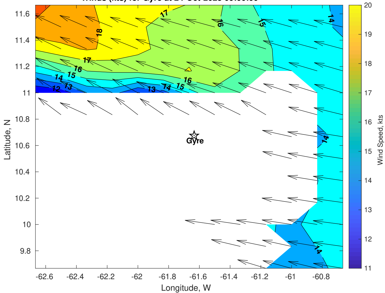
Winds (kts) for Gyre at 24-Oct-2025 09:00:00
