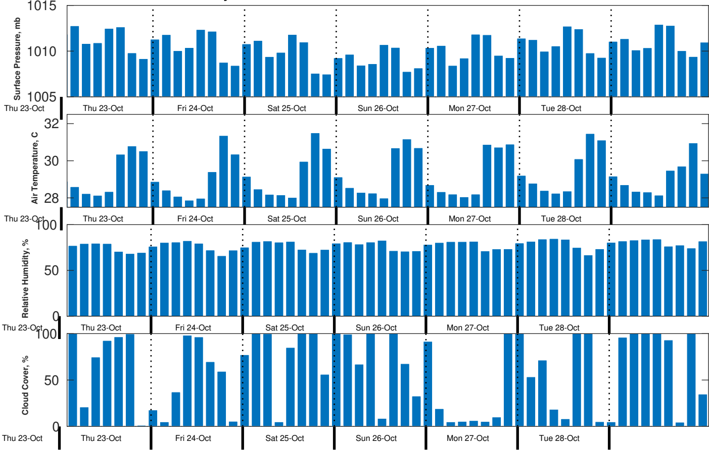
Met Forecast for Gyre from 23-Oct-2025 20:00:00 to 30-Oct-2025 20:00:00
