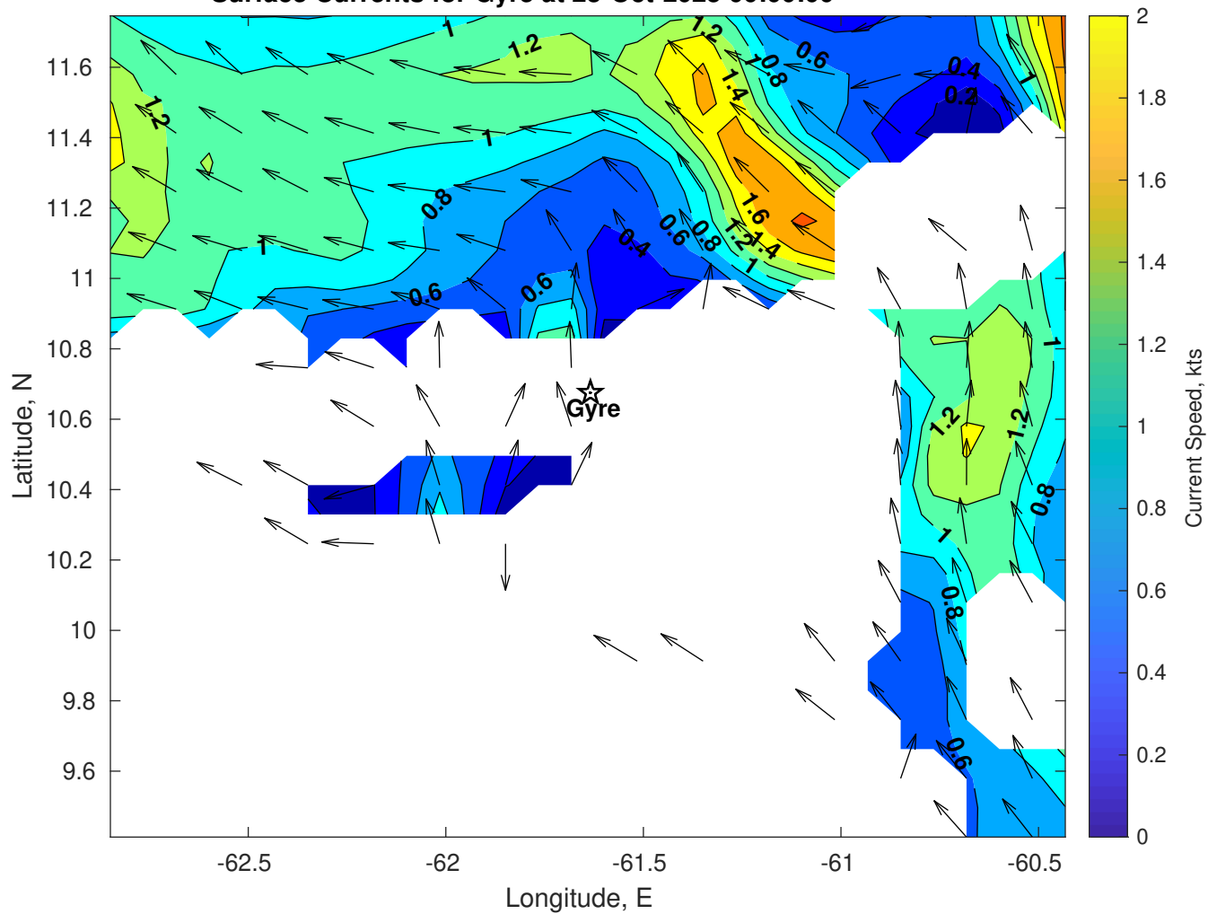
Surface Currents for Gyre at 23-Oct-2025 00:00:00
