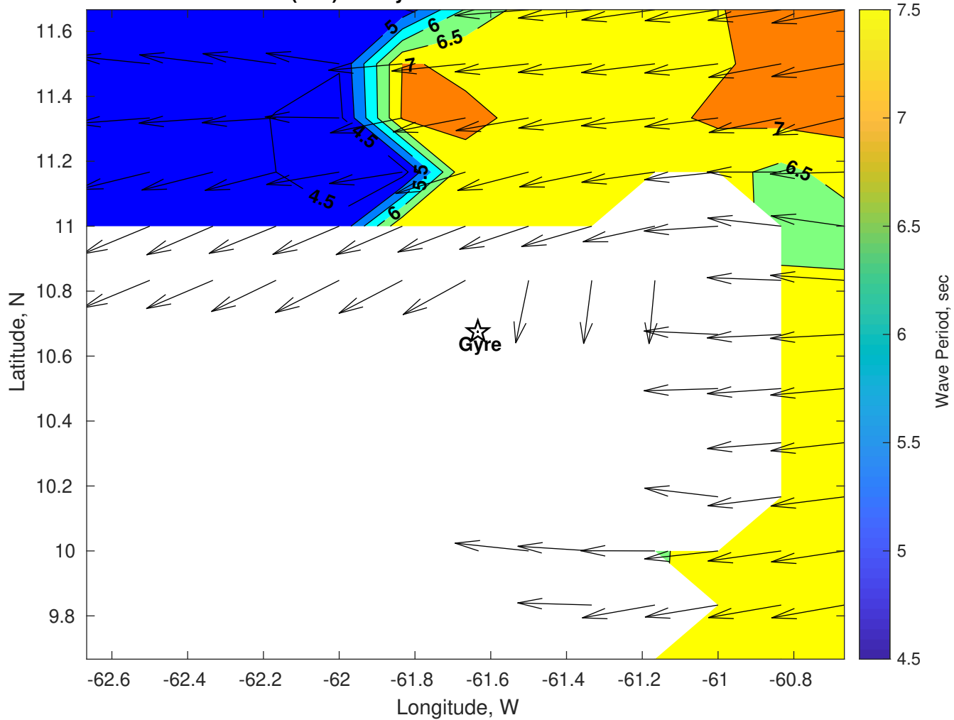
Wave Period (sec) for Gyre at 24-Oct-2025 09:00:00
