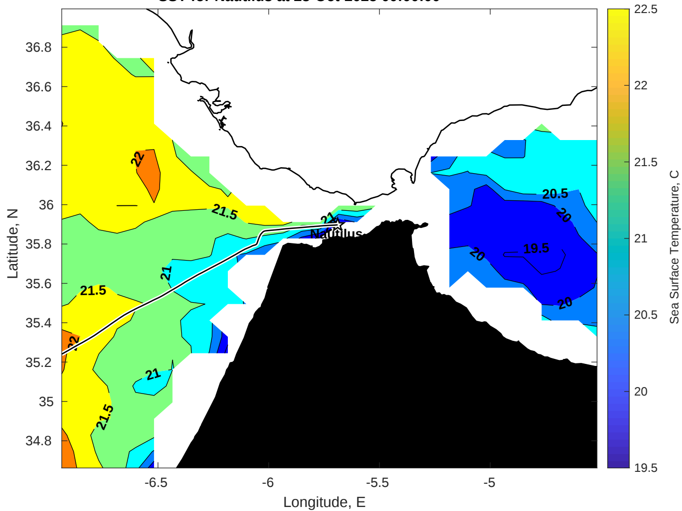
SST for Nautilus at 23-Oct-2025 00:00:00
