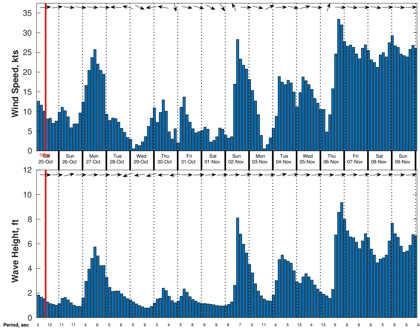
Wind & Wave Forecast for Nautilus from 24-Oct-2025 02:00:00 to 09-Nov-2025 02:00:00
