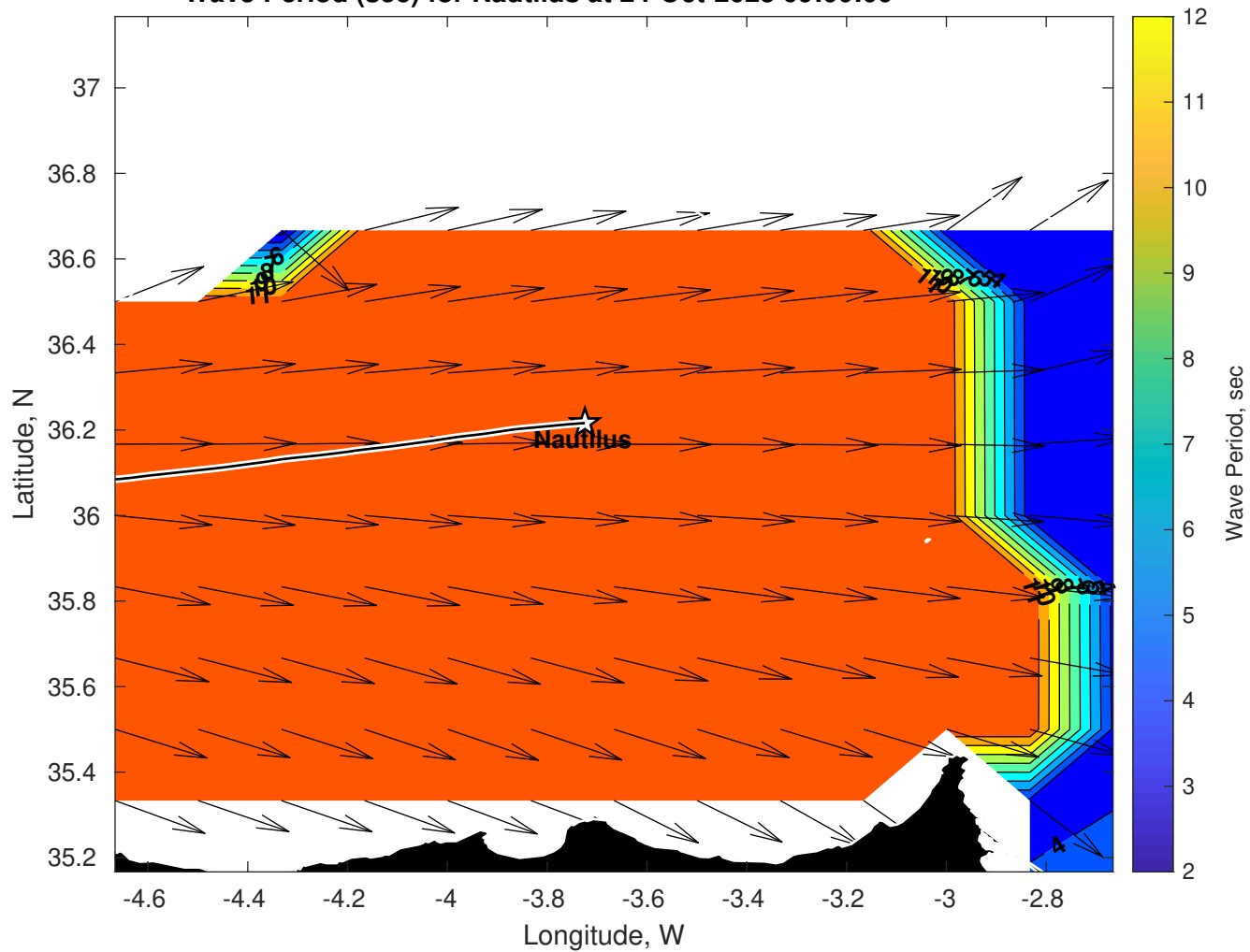
Wave Period (sec) for Nautilus at 24-Oct-2025 09:00:00
