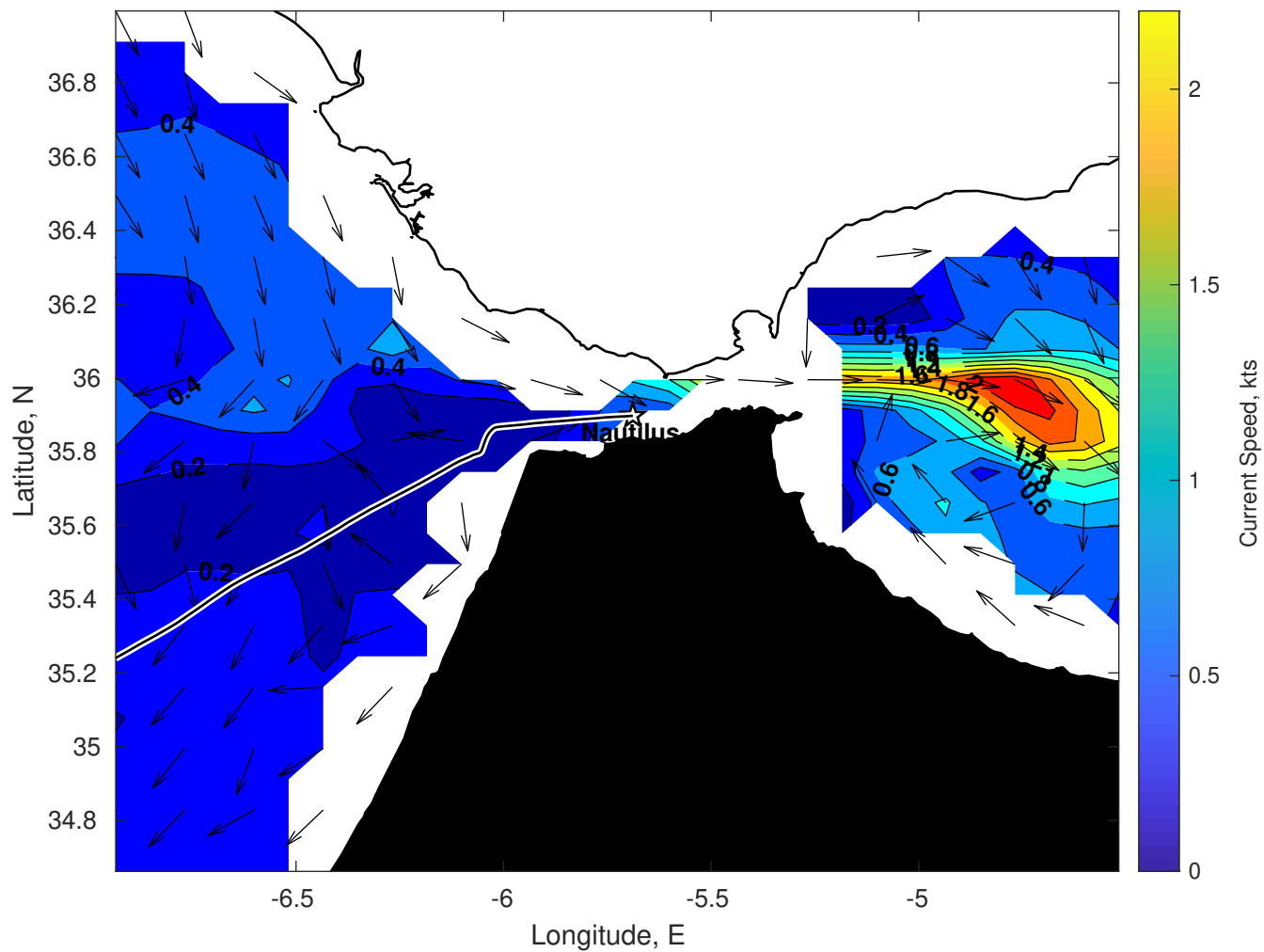
Surface Currents for Nautilus at 23-Oct-2025 00:00:00
