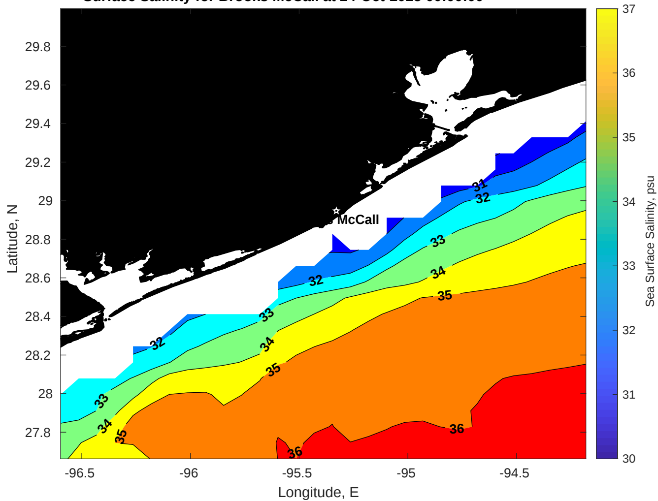
Surface Salinity for Brooks McCall at 24-Oct-2025 00:00:00
