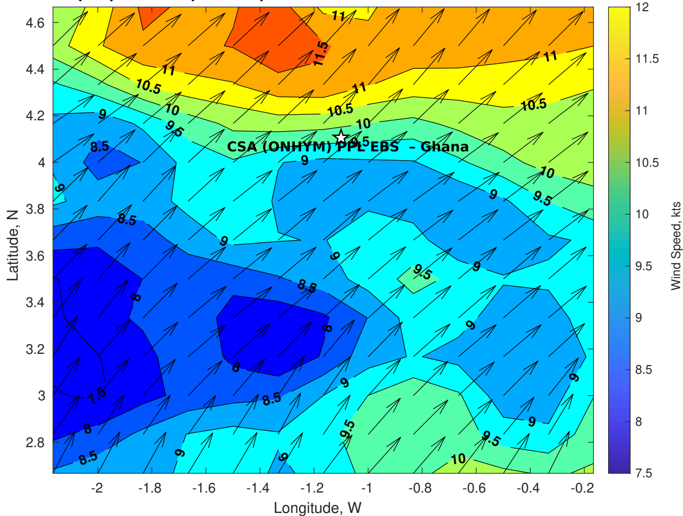
Winds (kts) for CSA (ONHYM) PPL EBS - Ghana at 22-Oct-2025 21:00:00
