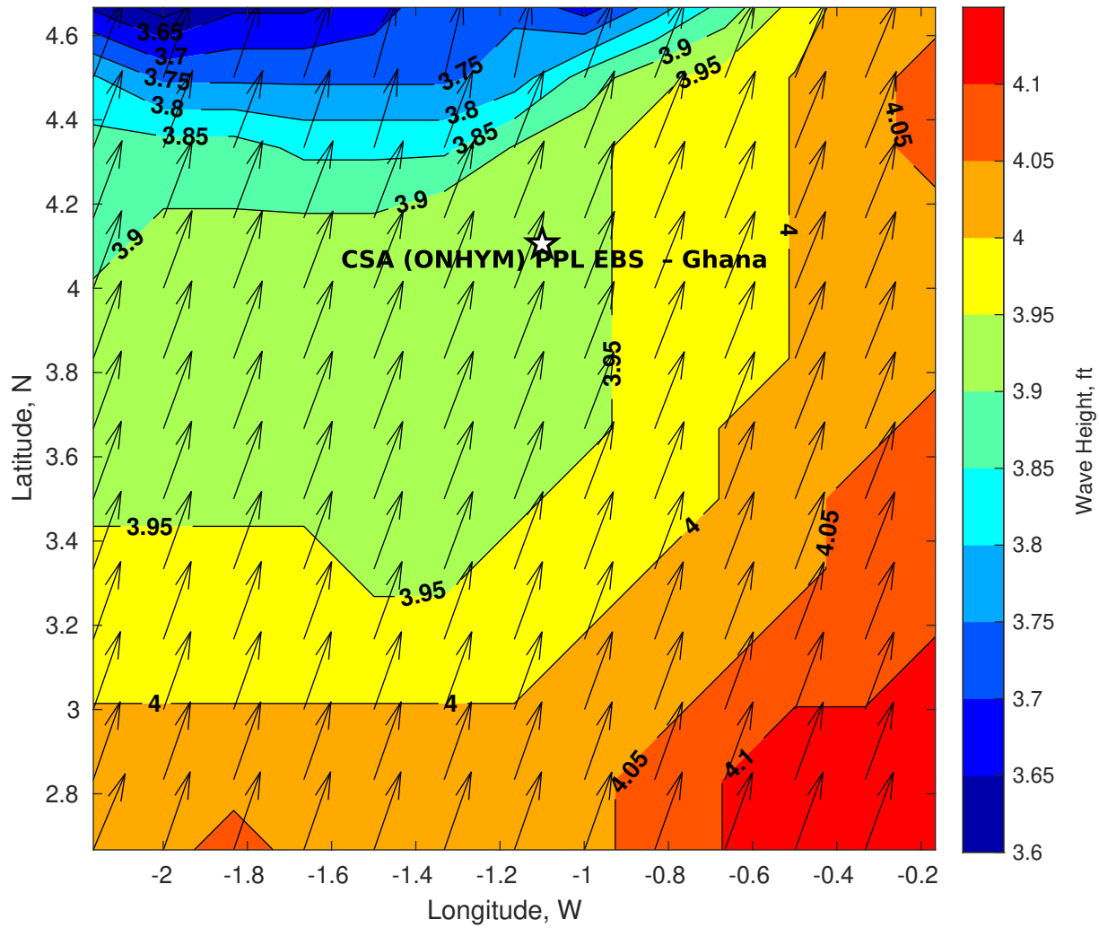
Wave Height (ft) for CSA (ONHYM) PPL EBS - Ghana at 22-Oct-2025 21:00:00
