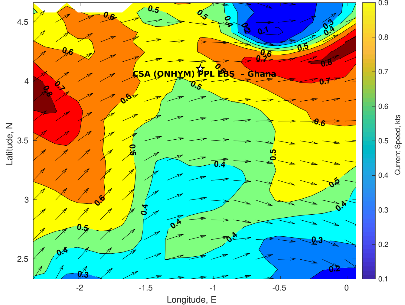
Surface Currents for CSA (ONHYM) PPL EBS - Ghana at 22-Oct-2025 00:00:00
