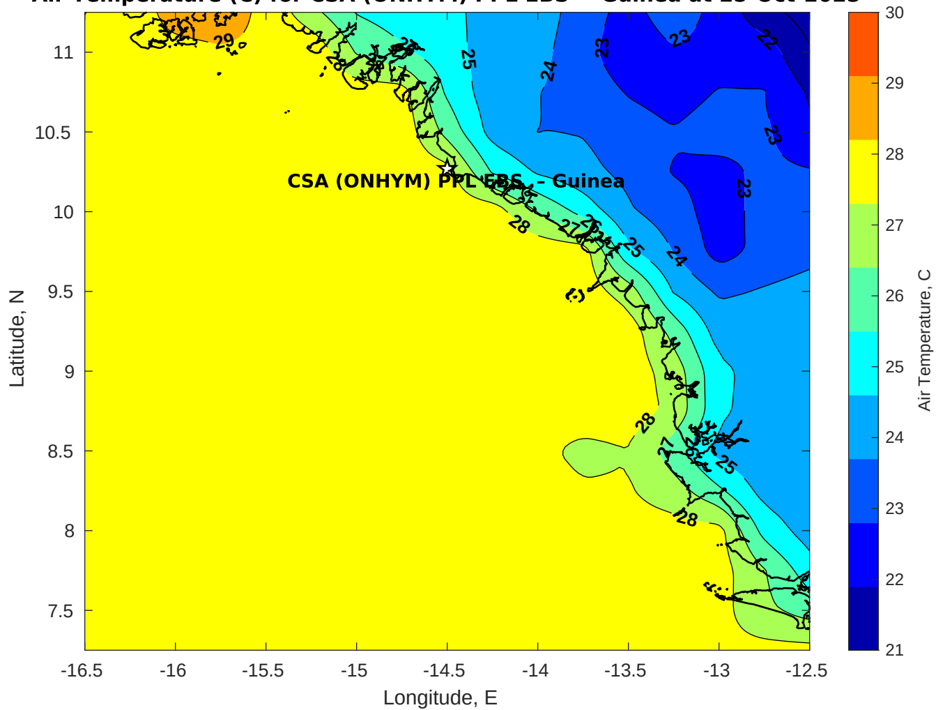
Air Temperature (C) for CSA (ONHYM) PPL EBS - Guinea at 25-Oct-2025
