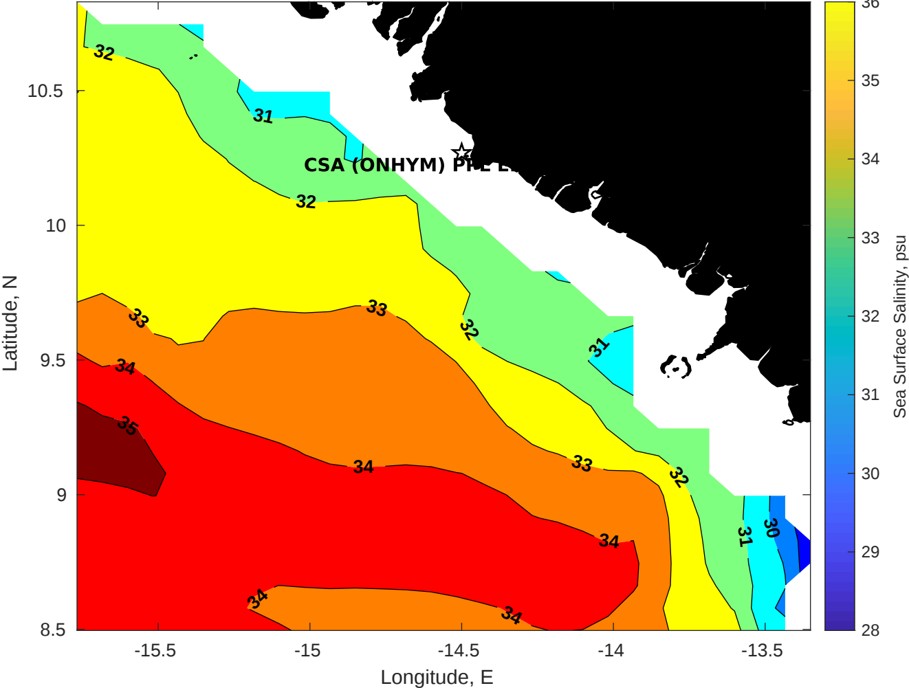
Surface Salinity for CSA (ONHYM) PPL EBS - Guinea at 22-Oct-2025 00:00:00
