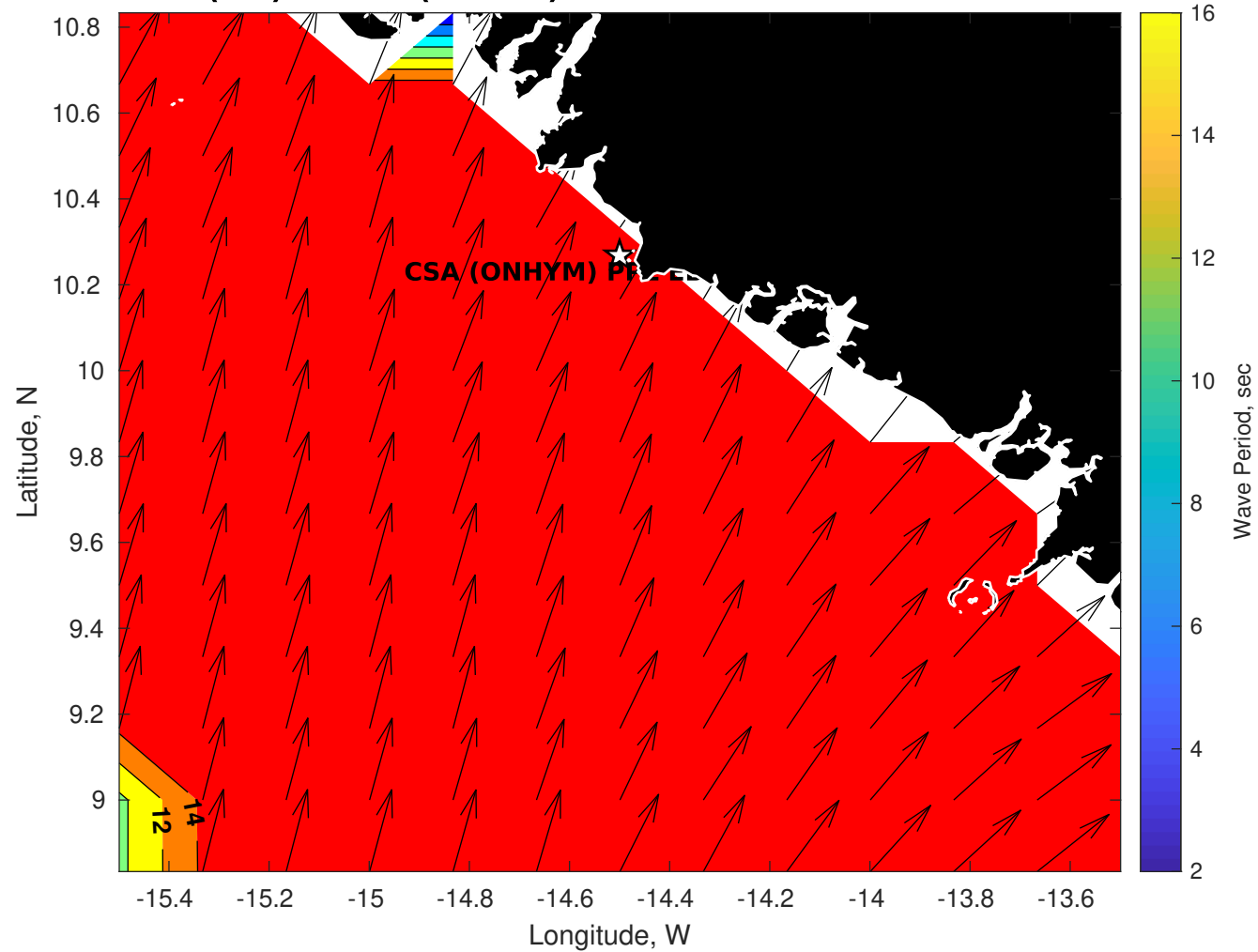
Wave Period (sec) for CSA (ONHYM) PPL EBS - Guinea at 22-Oct-2025 21:00:00
