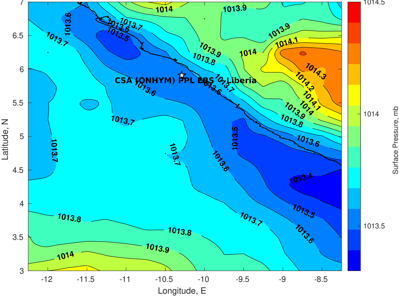
Surface Pressure (mb) for CSA (ONHYM) PPL EBS - Liberia at 27-Oct-2025 00:00:00
