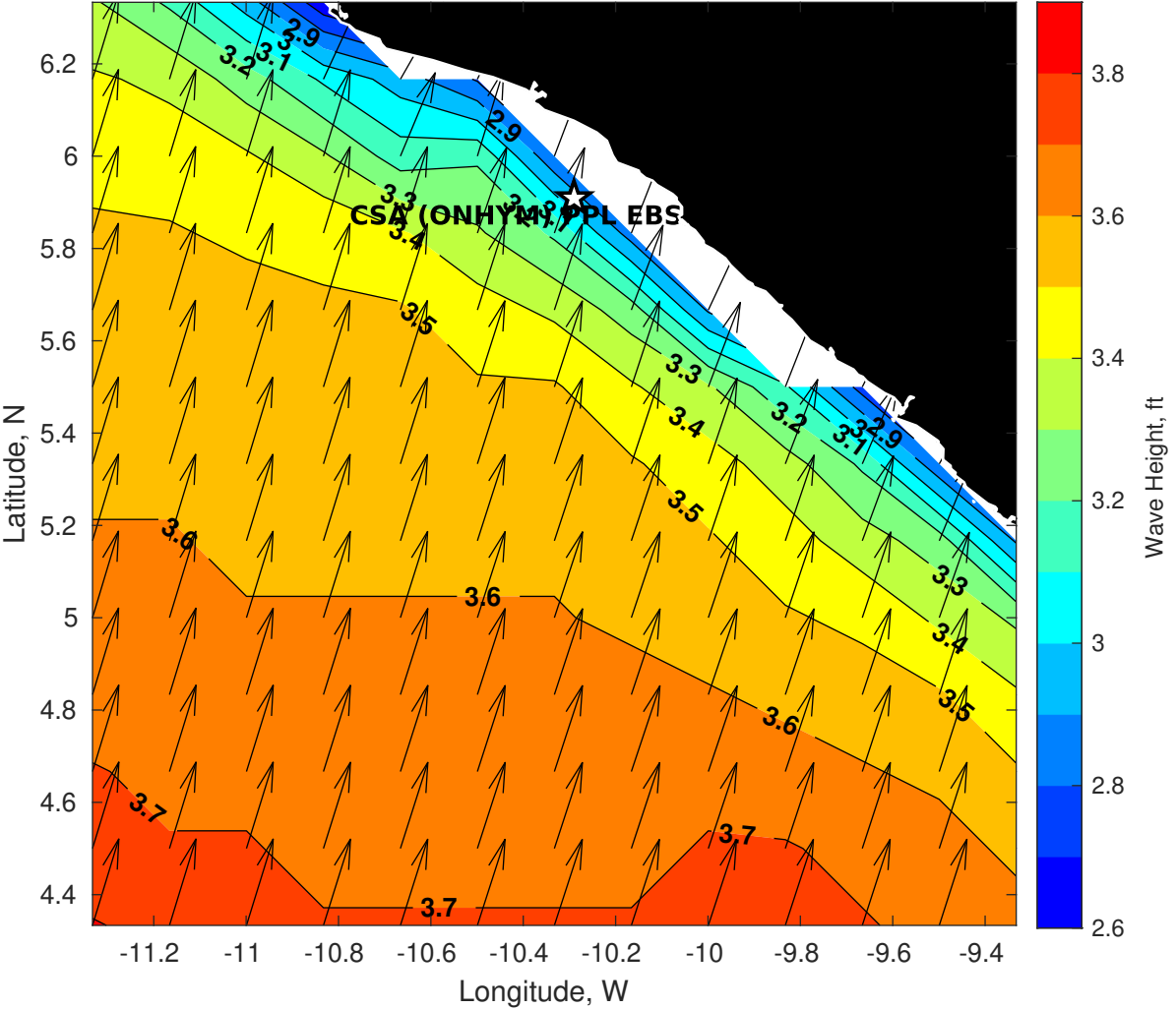
Wave Height (ft) for CSA (ONHYM) PPL EBS - Liberia at 22-Oct-2025 21:00:00
