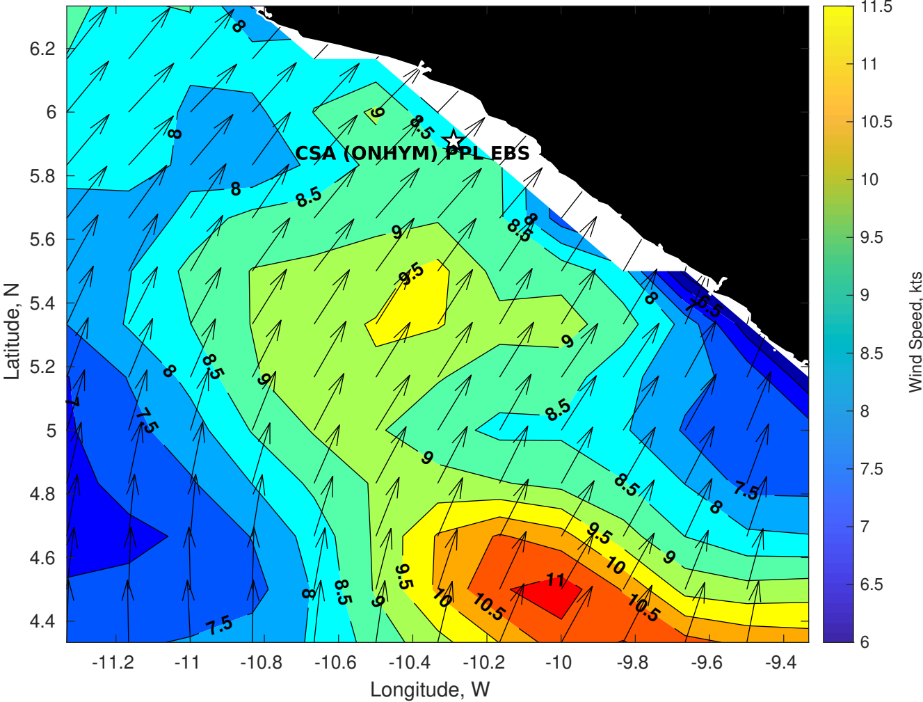
Winds (kts) for CSA (ONHYM) PPL EBS - Liberia at 22-Oct-2025 21:00:00
