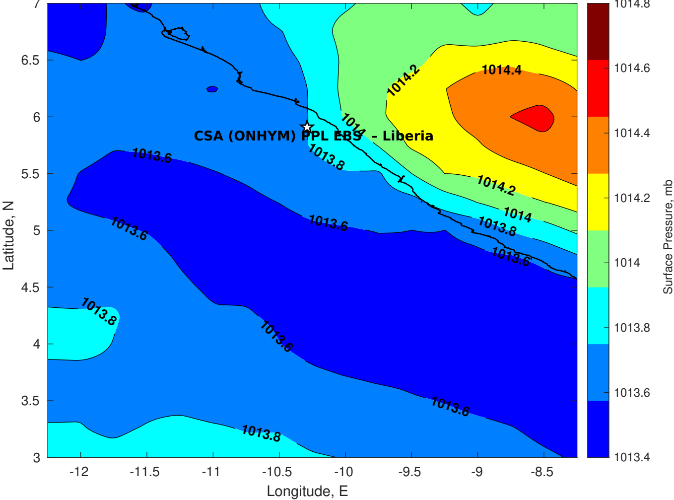
Surface Pressure (mb) for CSA (ONHYM) PPL EBS - Liberia at 26-Oct-2025 00:00:00
