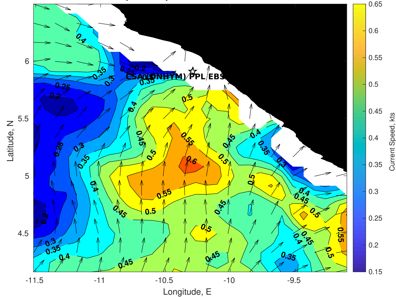
Surface Currents for CSA (ONHYM) PPL EBS - Liberia at 22-Oct-2025 00:00:00
