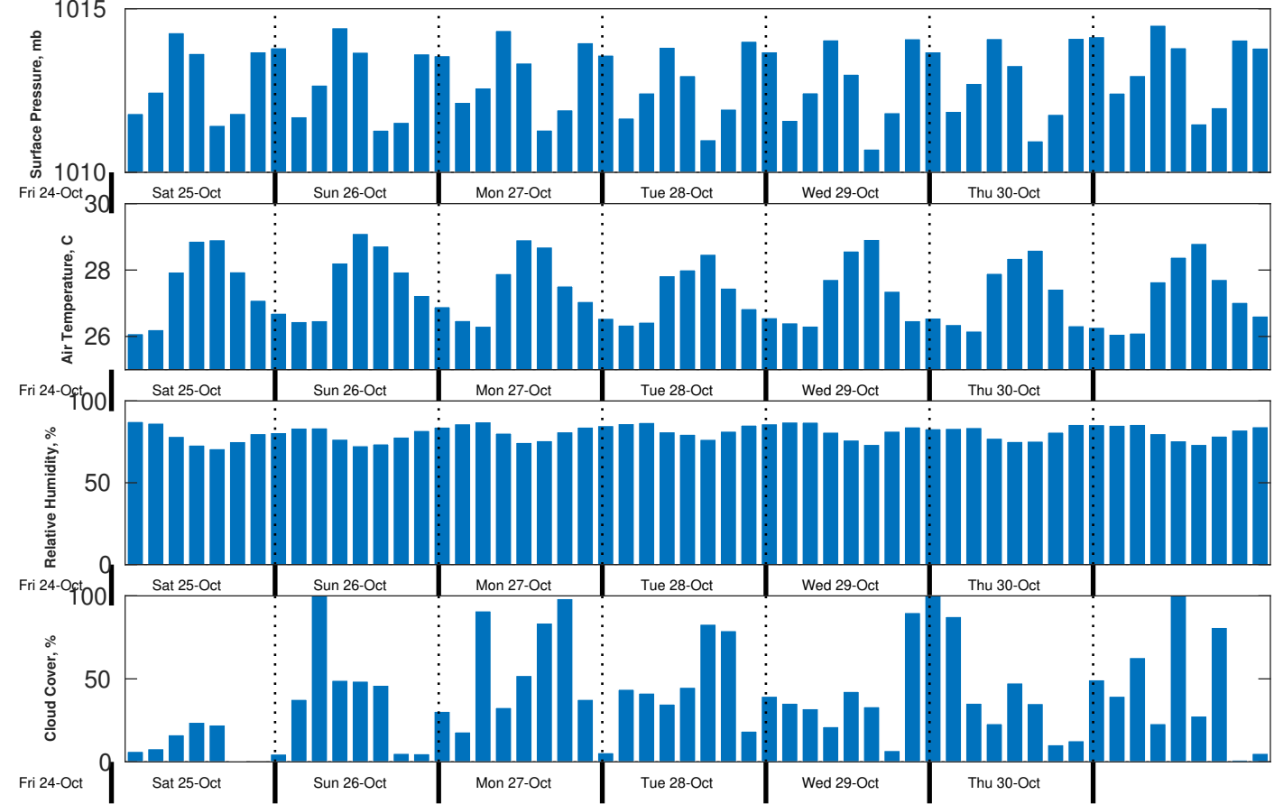
Met Forecast for CSA (ONHYM) PPL EBS - Liberia from 25-Oct-2025 00:00:00 to 01-Nov-2025 00:00:00
