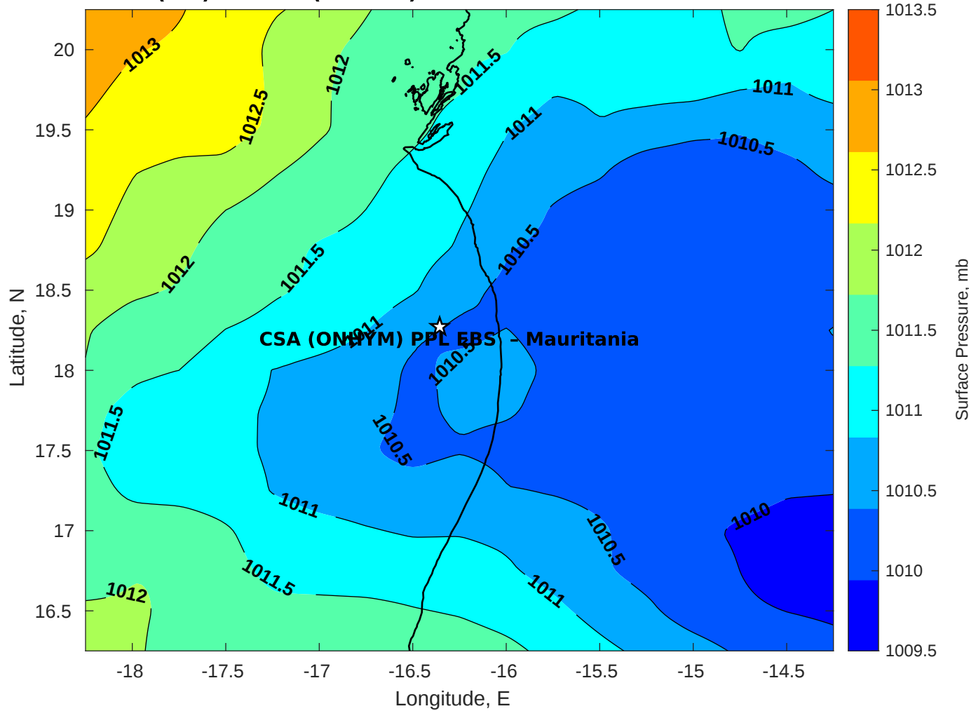
Surface Pressure (mb) for CSA (ONHYM) PPL EBS - Mauritania at 26-Oct-2025 00:00:00
