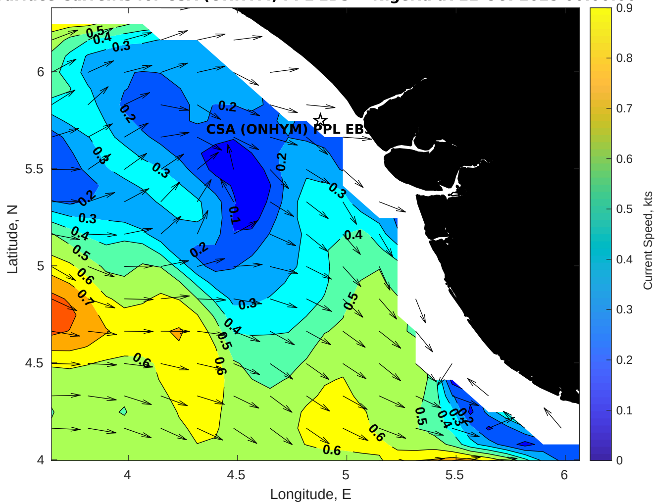
Surface Currents for CSA (ONHYM) PPL EBS - Nigeria at 22-Oct-2025 00:00:00
