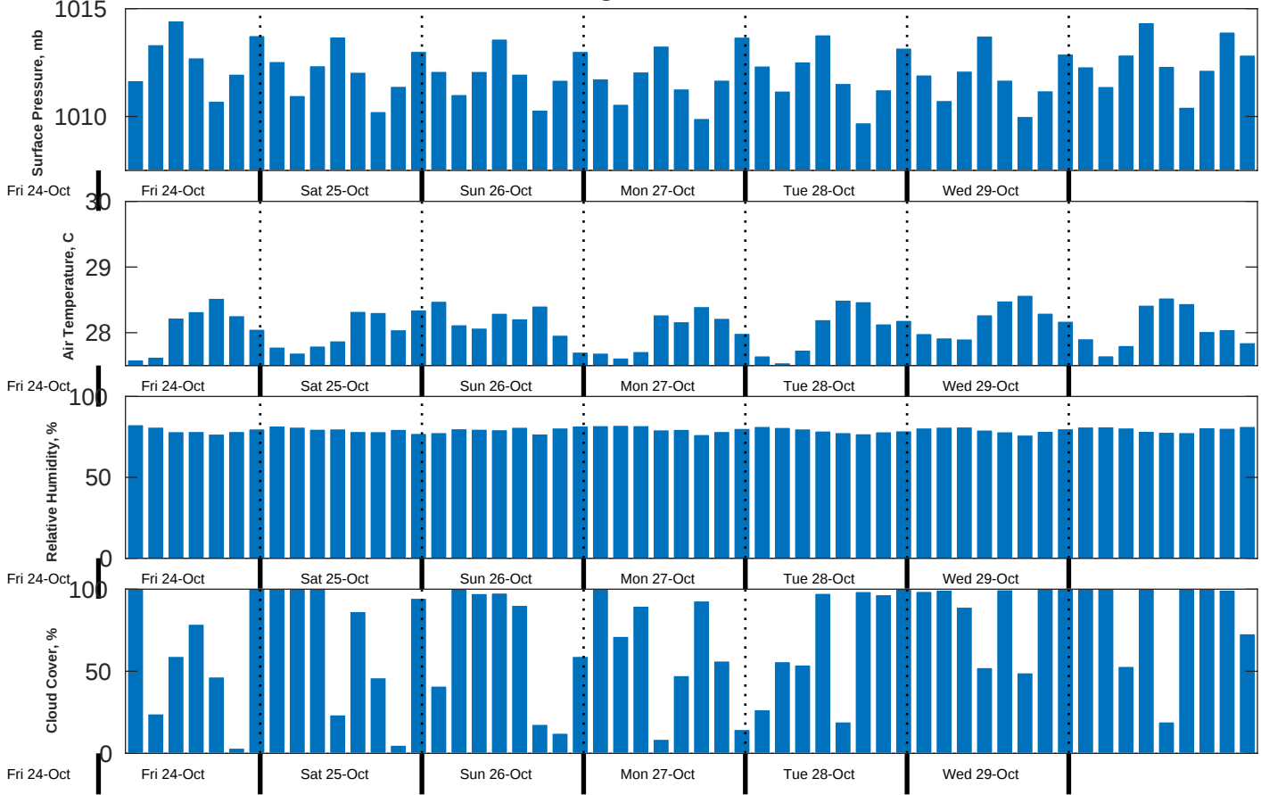
Met Forecast for CSA (ONHYM) PPL EBS - Nigeria from 25-Oct-2025 00:00:00 to 01-Nov-2025 00:00:00
