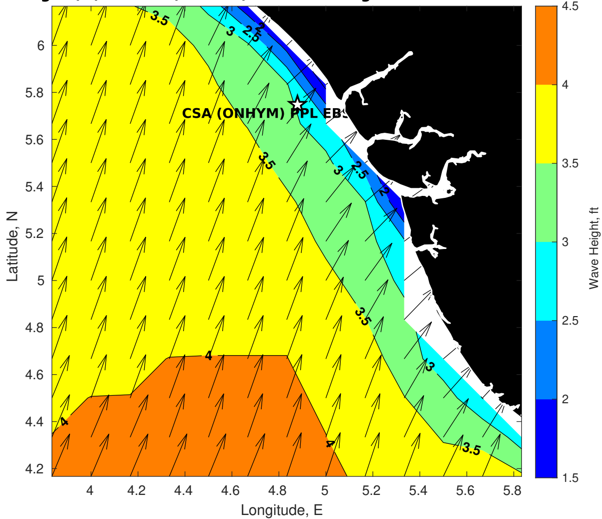
Wave Height (ft) for CSA (ONHYM) PPL EBS - Nigeria at 22-Oct-2025 21:00:00
