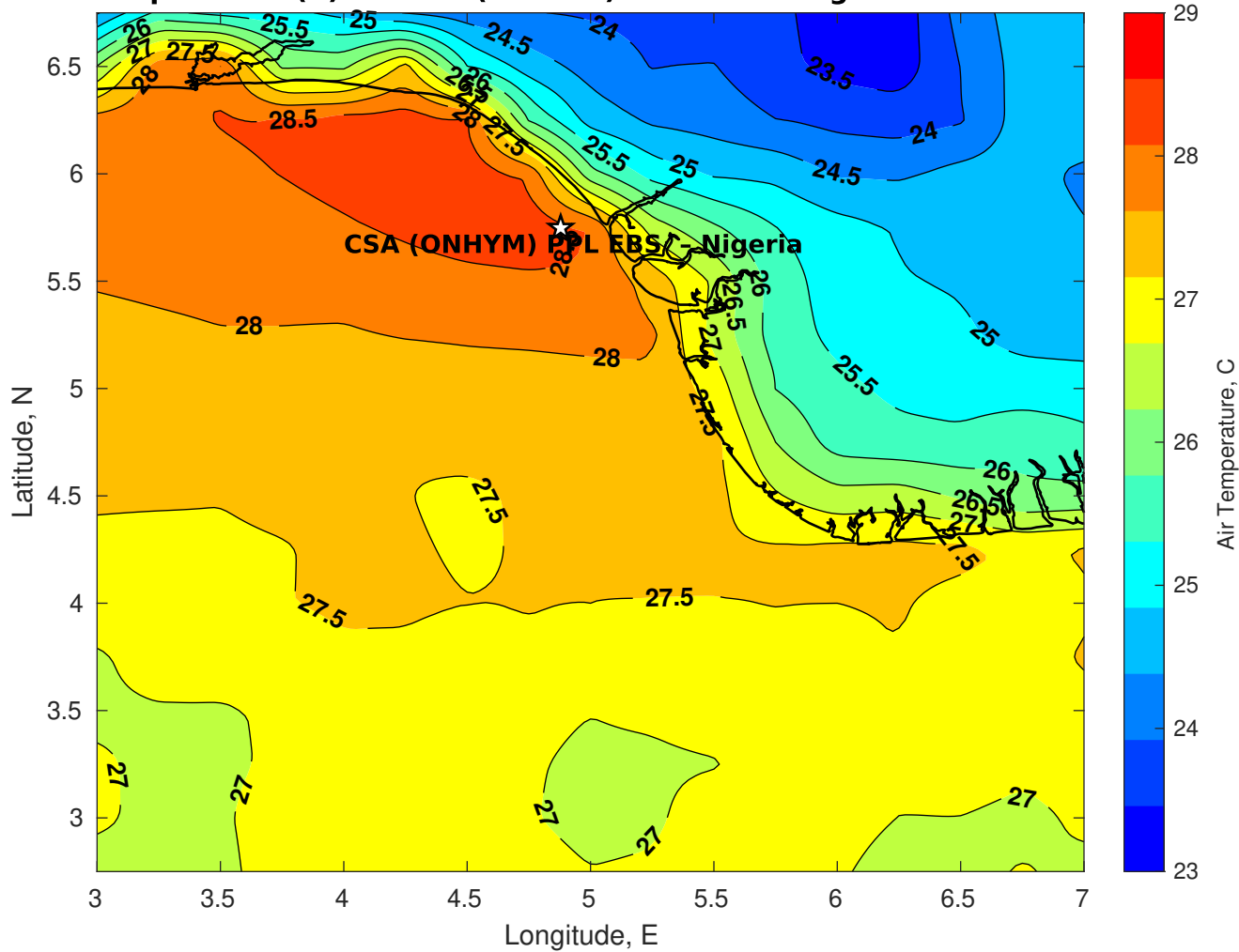
Air Temperature (C) for CSA (ONHYM) PPL EBS - Nigeria at 25-Oct-2025
