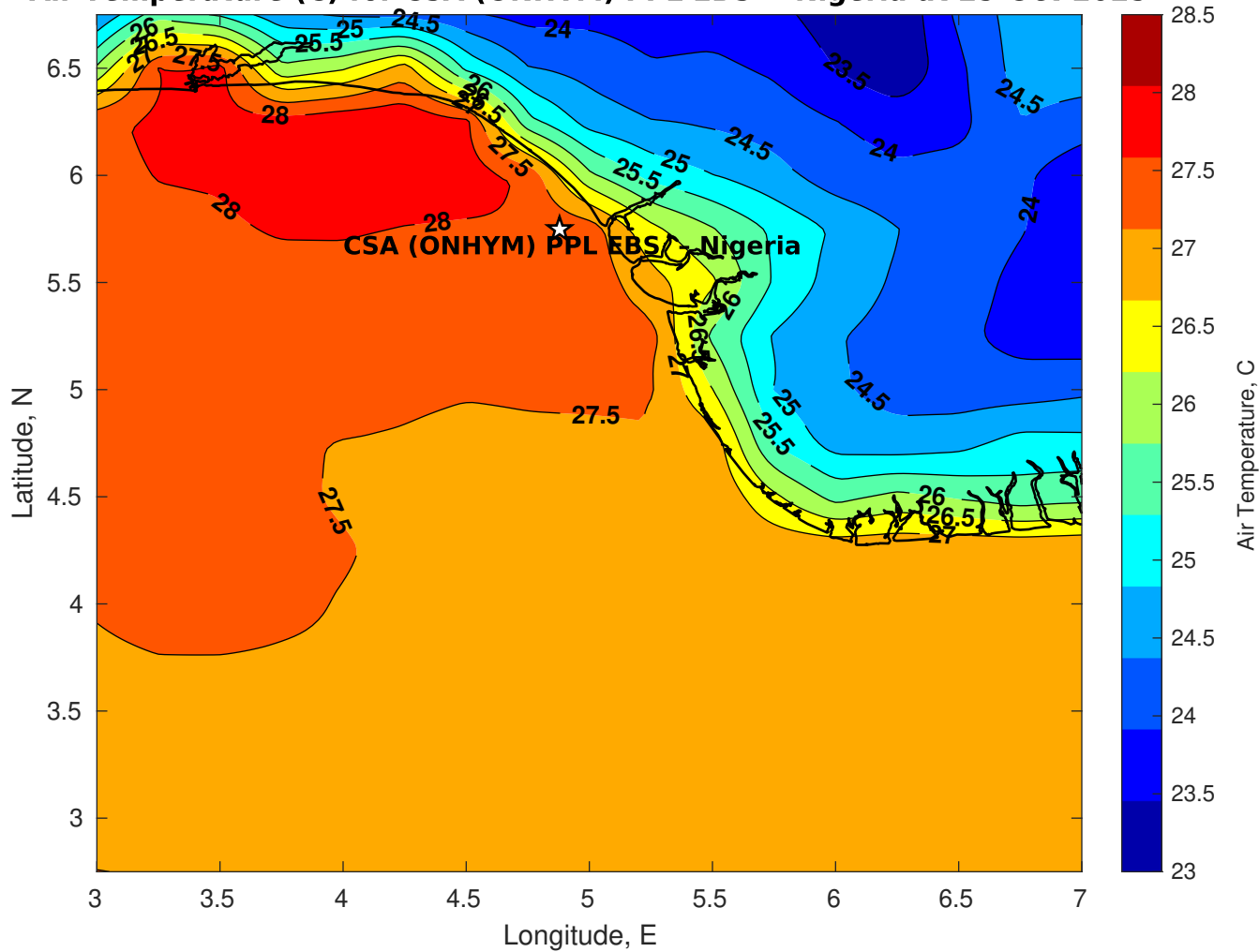
Air Temperature (C) for CSA (ONHYM) PPL EBS - Nigeria at 25-Oct-2025
