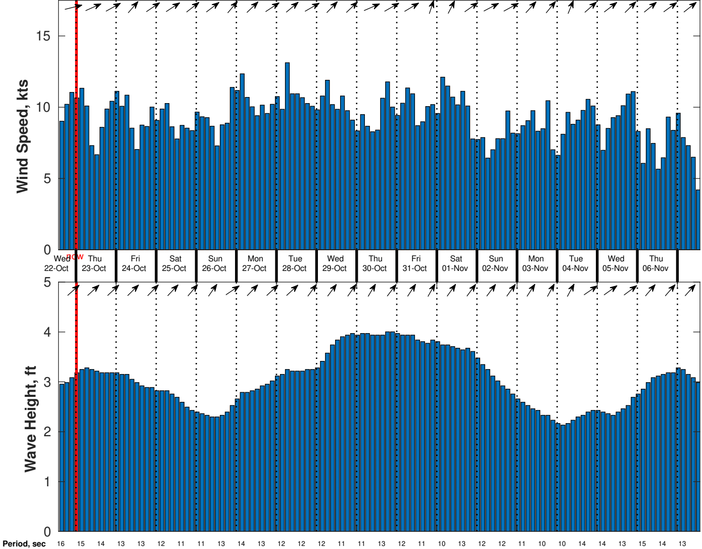
Wind & Wave Forecast for CSA (ONHYM) PPL EBS - Nigeria from 22-Oct-2025 14:00:00 to 07-Nov-2025 14:00:00
