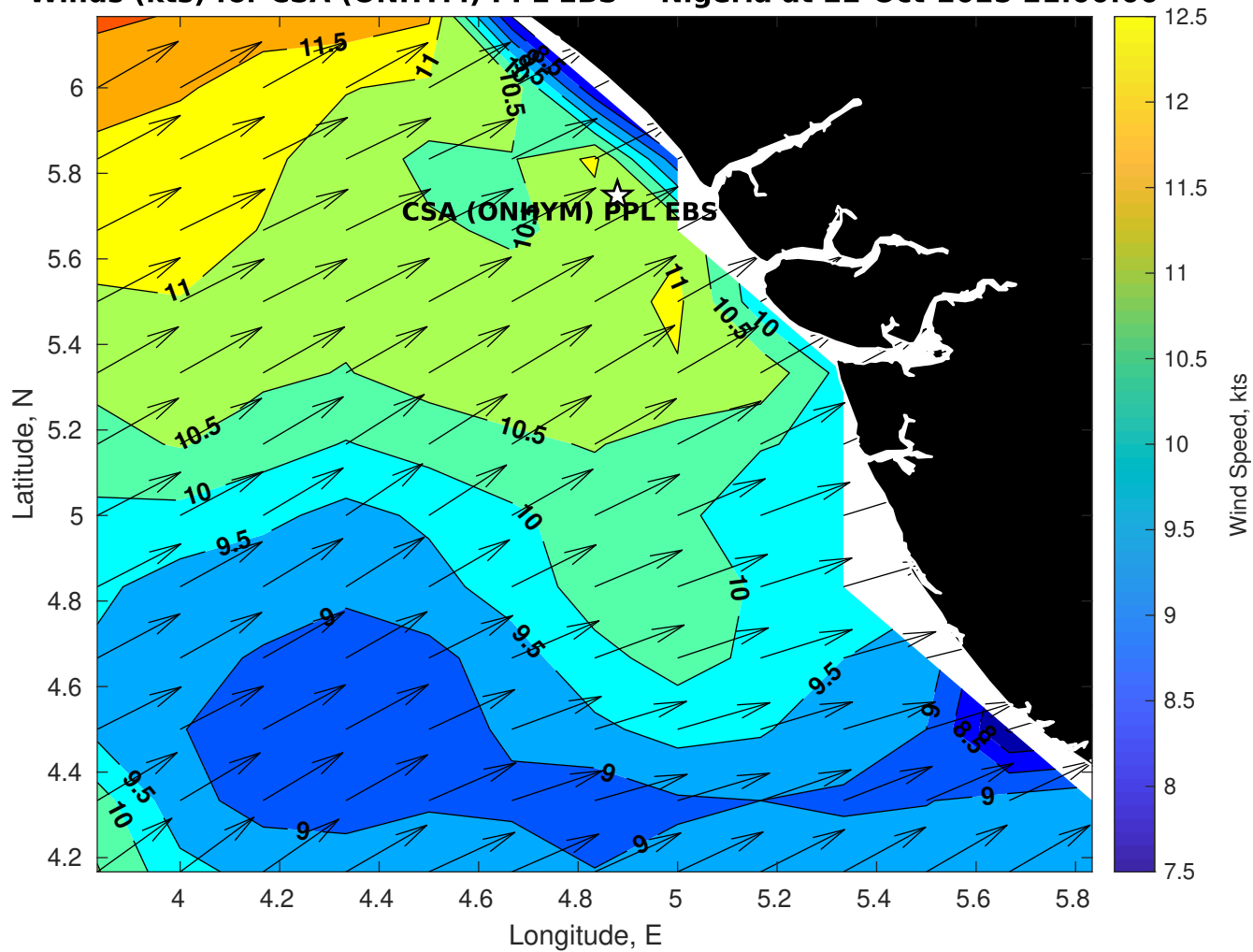
Winds (kts) for CSA (ONHYM) PPL EBS - Nigeria at 22-Oct-2025 21:00:00
