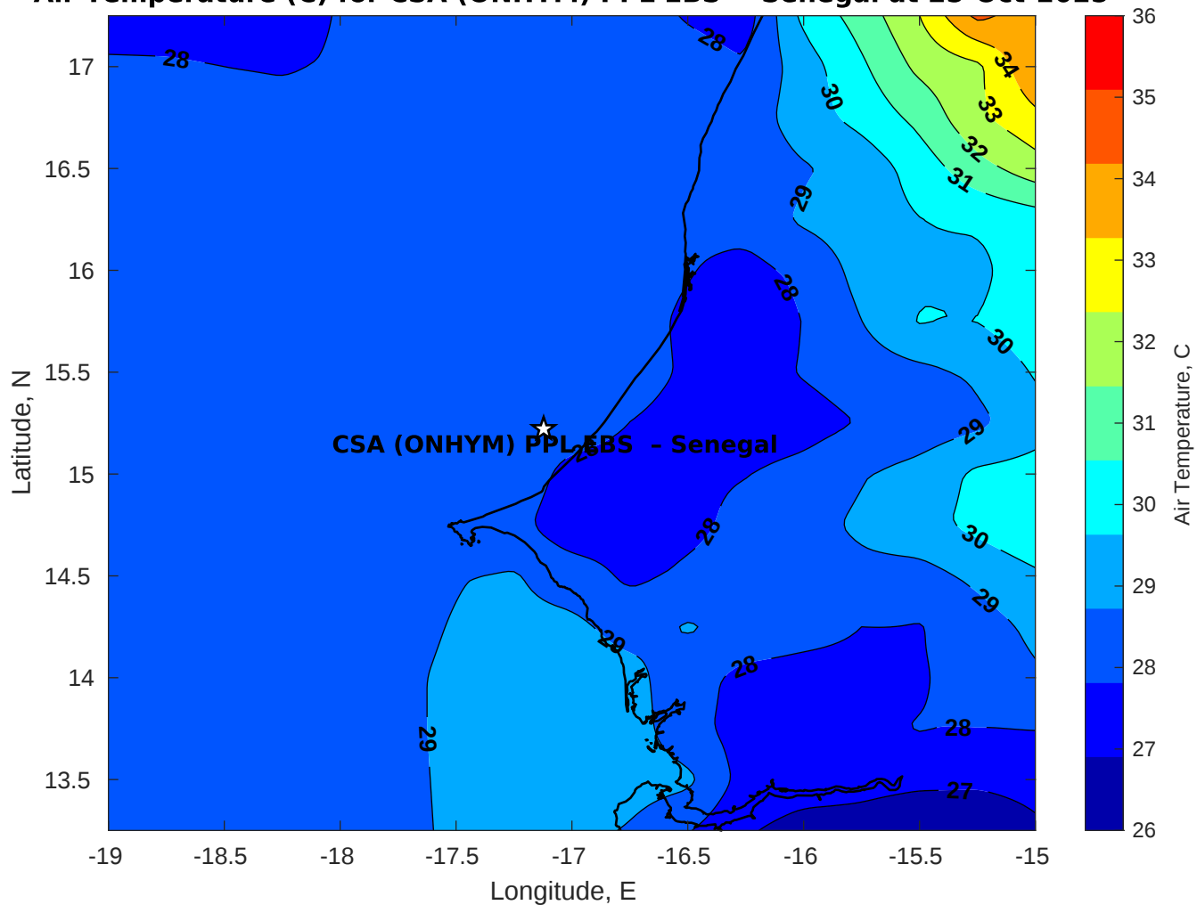
Air Temperature (C) for CSA (ONHYM) PPL EBS - Senegal at 25-Oct-2025
