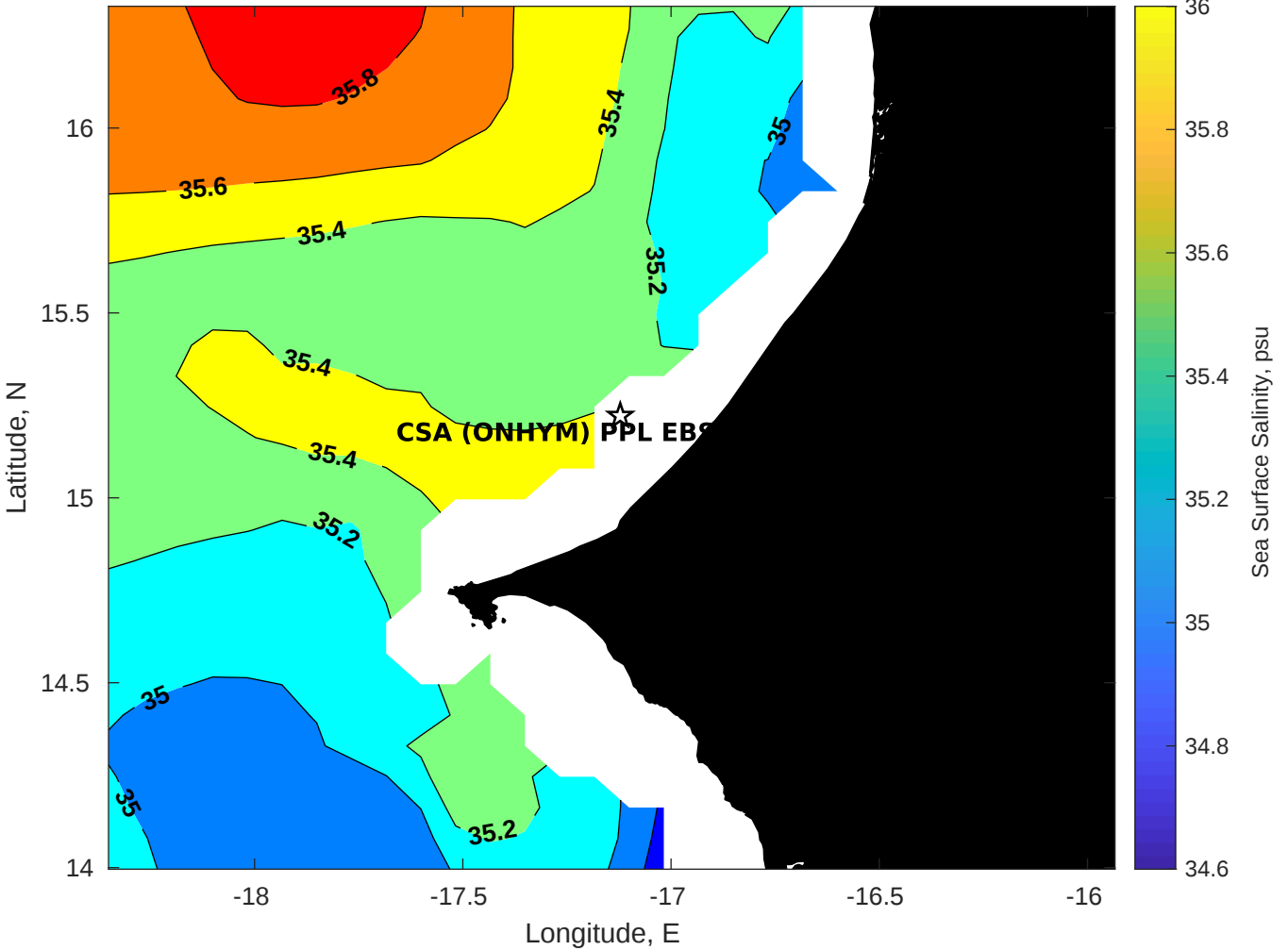
Surface Salinity for CSA (ONHYM) PPL EBS - Senegal at 22-Oct-2025 00:00:00
