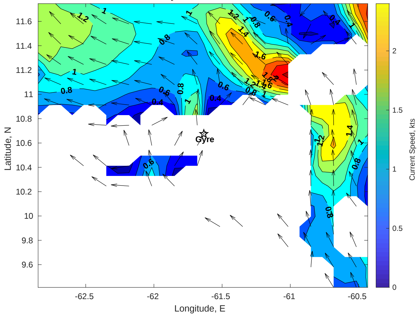
Surface Currents for Gyre at 24-Oct-2025 00:00:00
