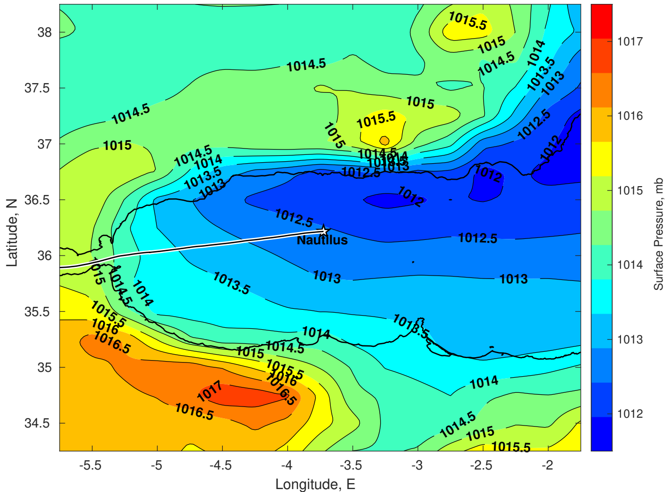
Surface Pressure (mb) for Nautilus at 26-Oct-2025 00:00:00
