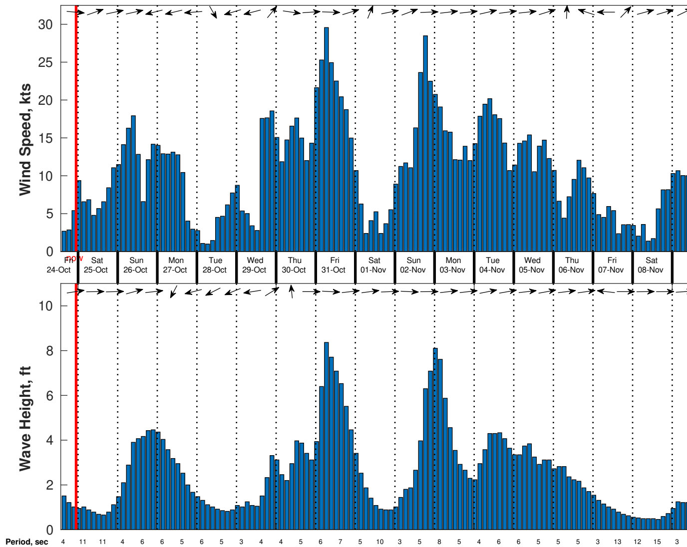
Wind & Wave Forecast for Nautilus from 24-Oct-2025 14:00:00 to 09-Nov-2025 14:00:00
