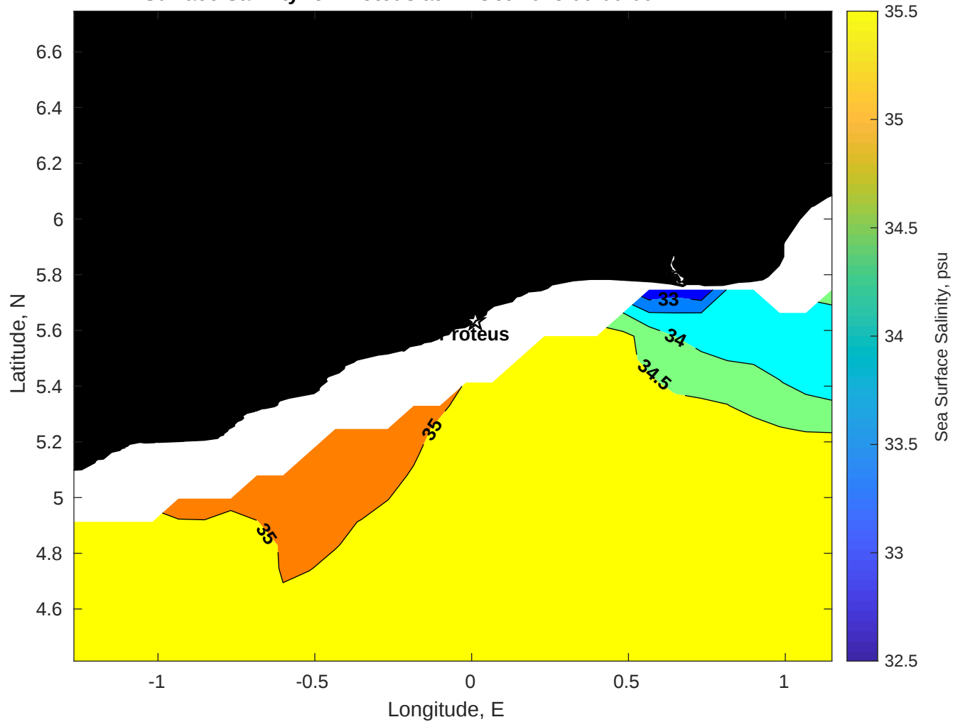
Surface Salinity for Proteus at 24-Oct-2025 00:00:00
