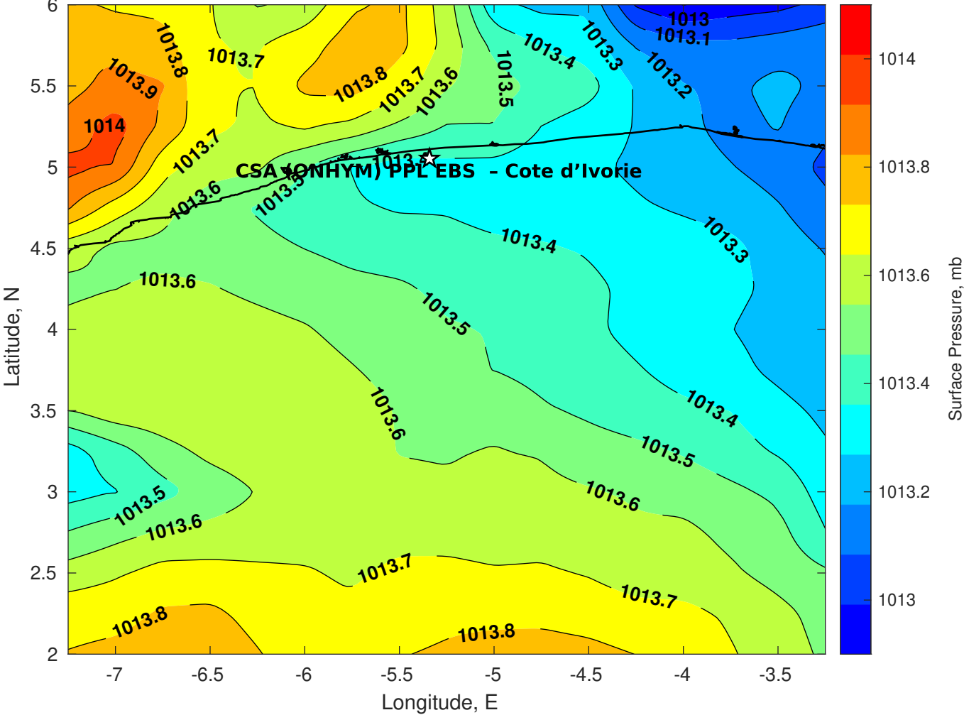
Surface Pressure (mb) for CSA (ONHYM) PPL EBS - Cote d'Ivoire at 28-Oct-2025 00:00:00
