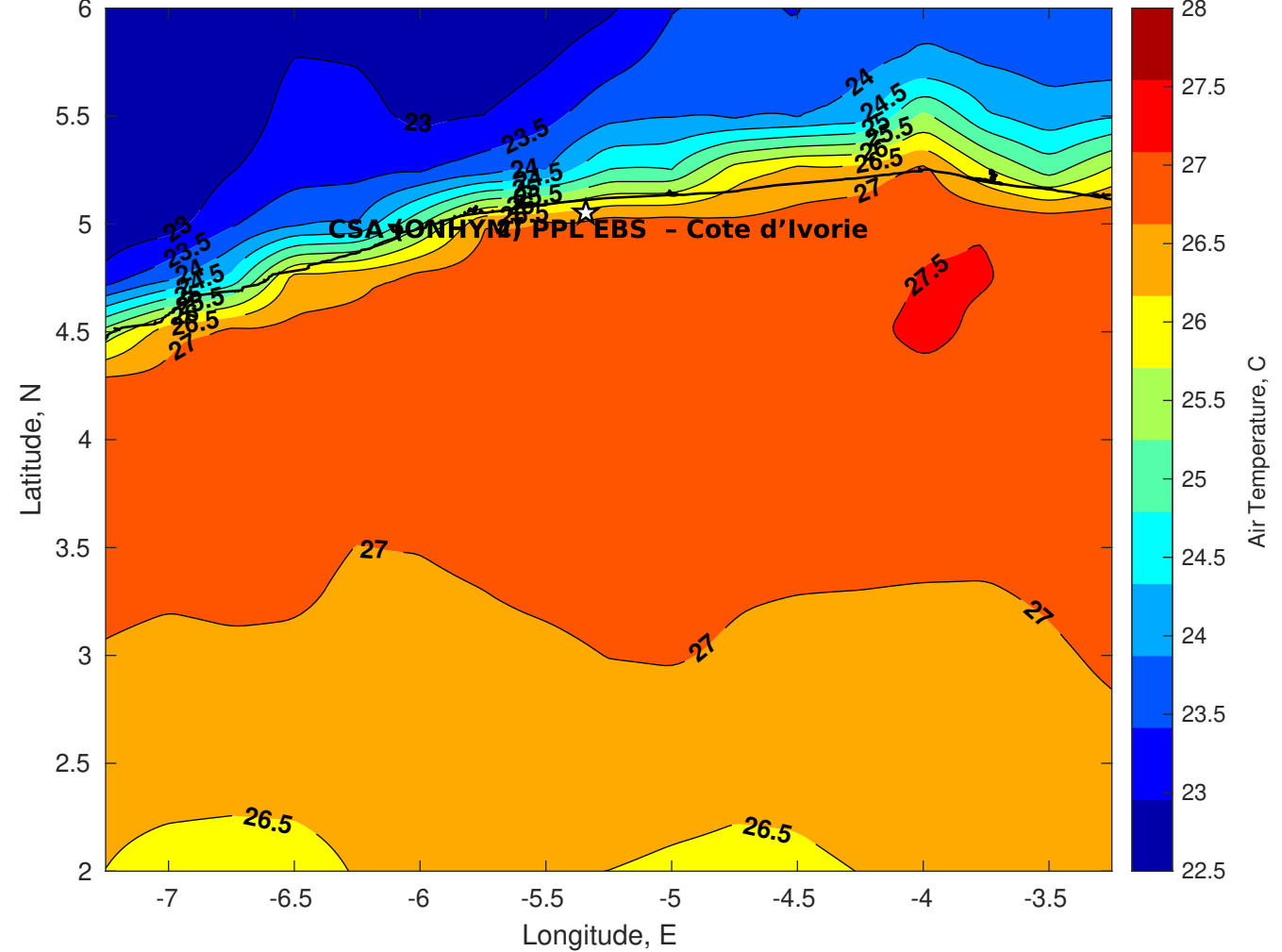
Air Temperature (C) for CSA (ONHYM) PPL EBS - Cote d'Ivoire at 26-Oct-2025
