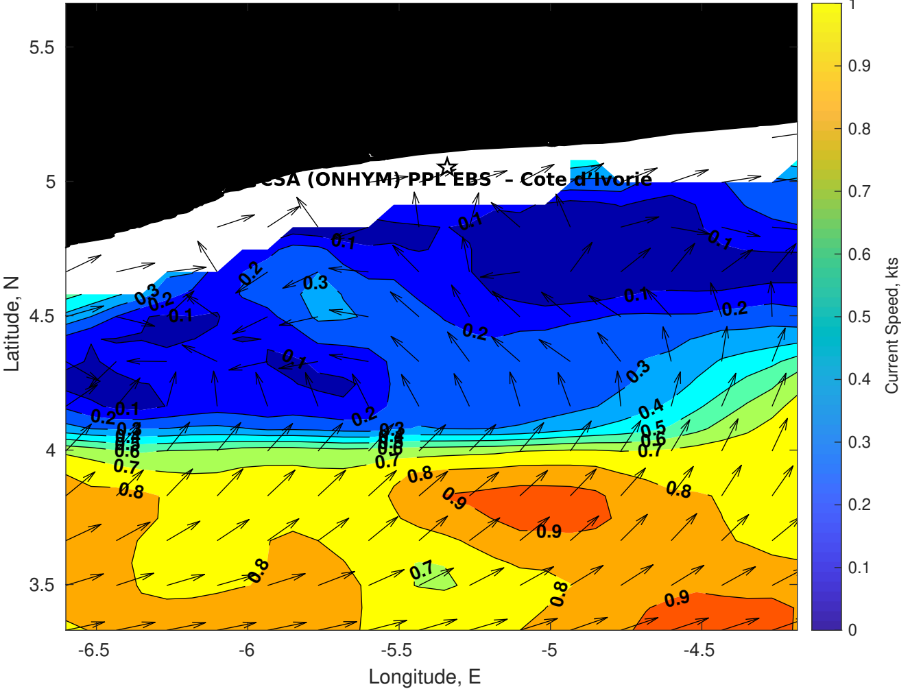
Surface Currents for CSA (ONHYM) PPL EBS - Cote d'Ivoire at 25-Oct-2025 00:00:00
