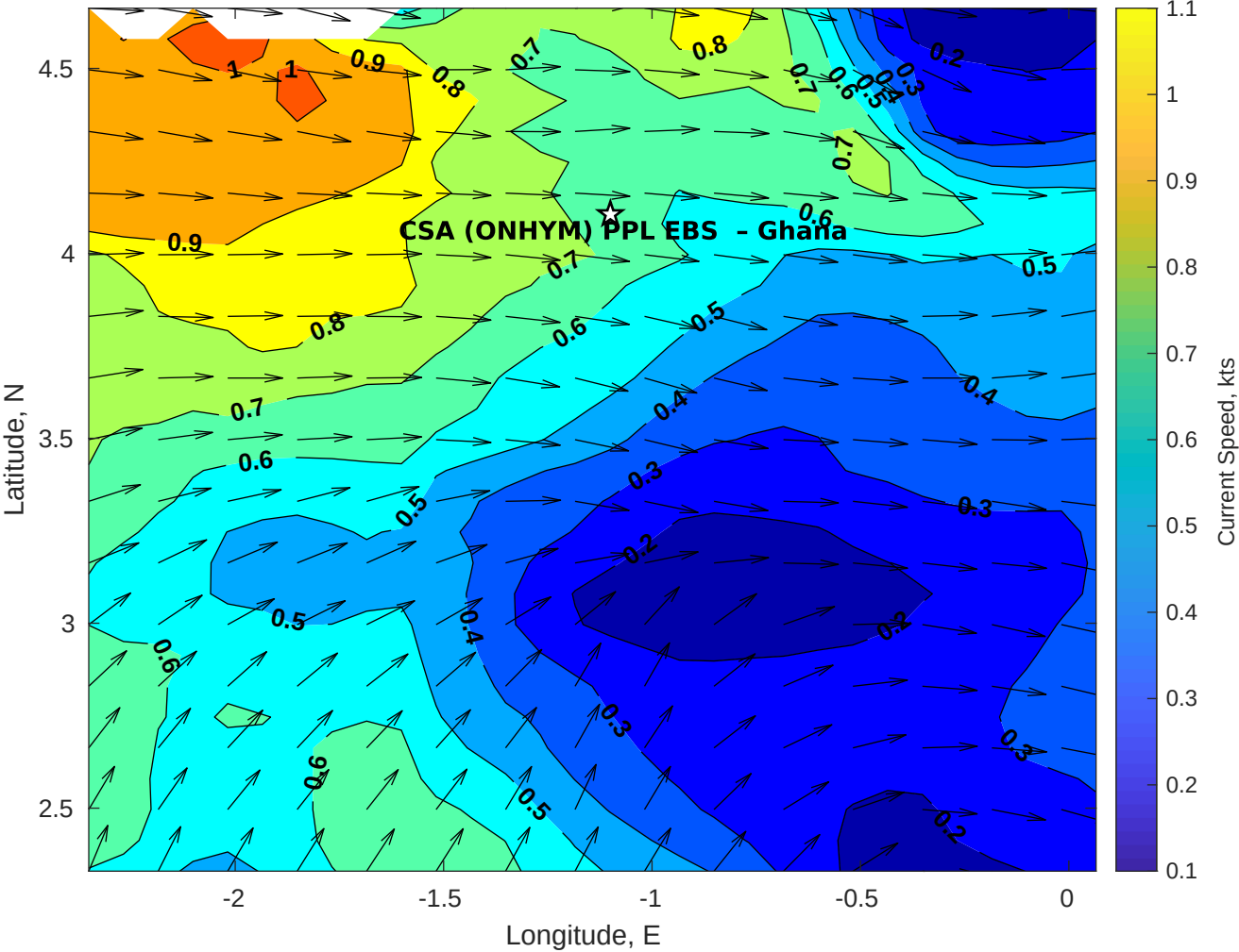
Surface Currents for CSA (ONHYM) PPL EBS - Ghana at 25-Oct-2025 00:00:00
