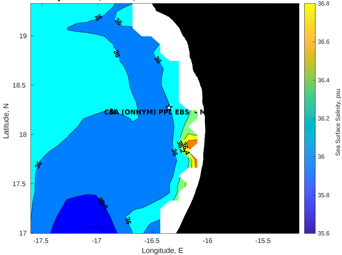
Surface Salinity for CSA (ONHYM) PPL EBS - Mauritania at 22-Oct-2025 00:00:00
