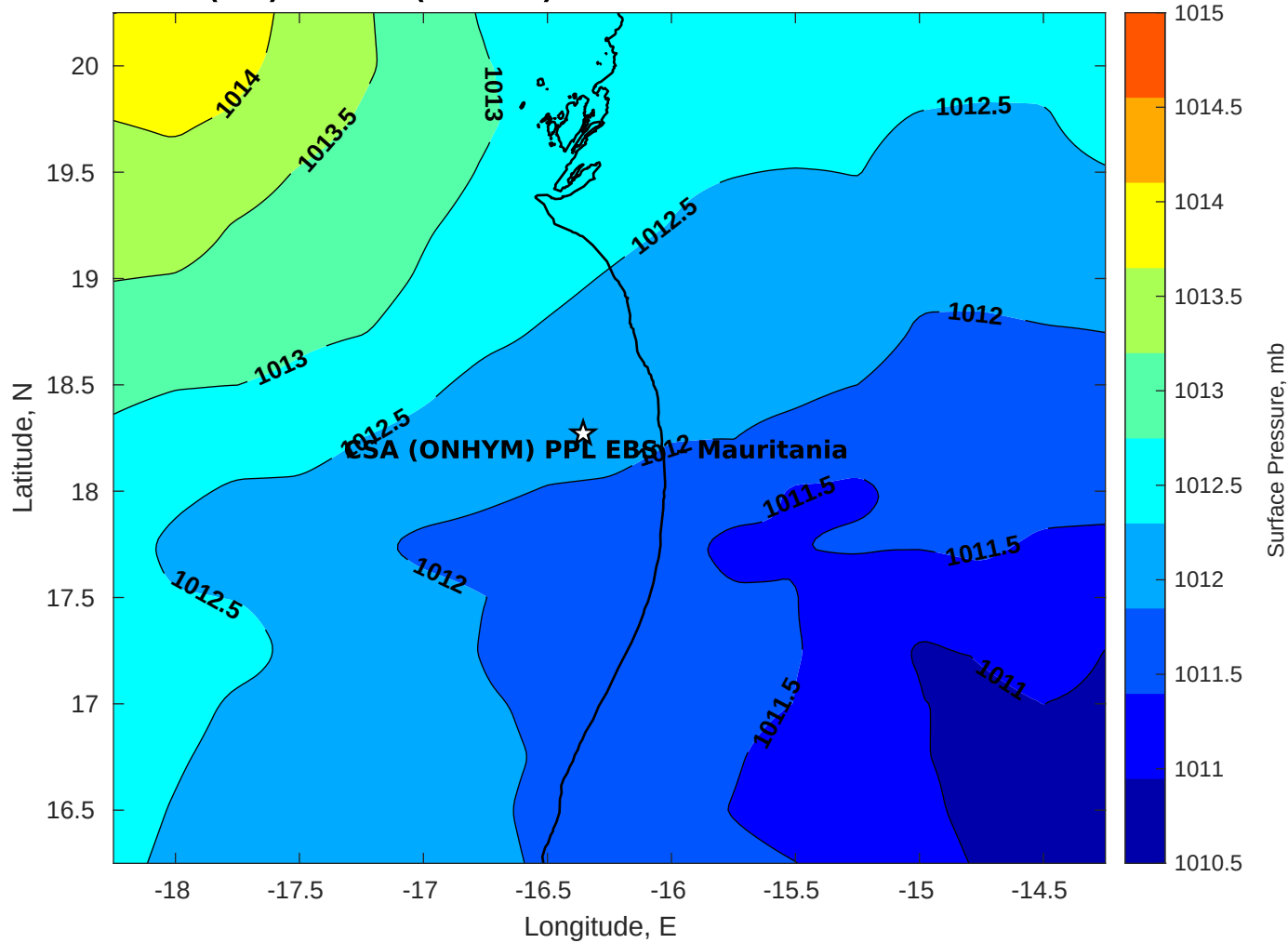
Surface Pressure (mb) for CSA (ONHYM) PPL EBS - Mauritania at 27-Oct-2025 00:00:00
