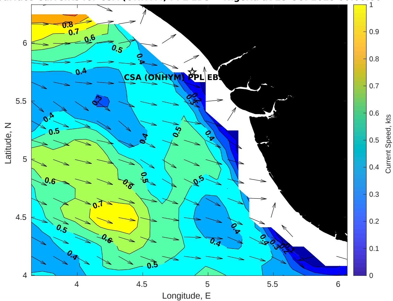
Surface Currents for CSA (ONHYM) PPL EBS - Nigeria at 25-Oct-2025 00:00:00
