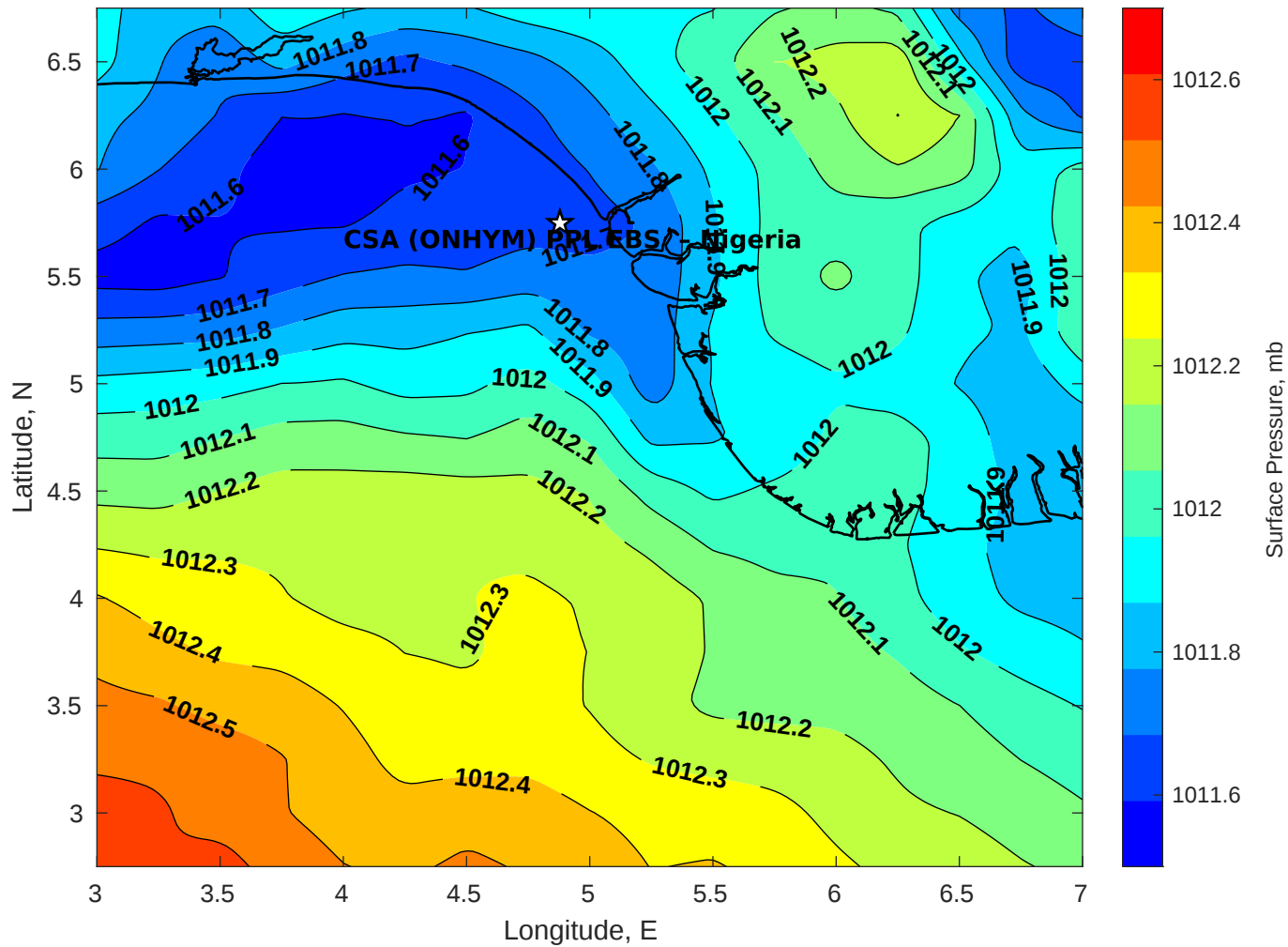
Surface Pressure (mb) for CSA (ONHYM) PPL EBS - Nigeria at 27-Oct-2025 00:00:00
