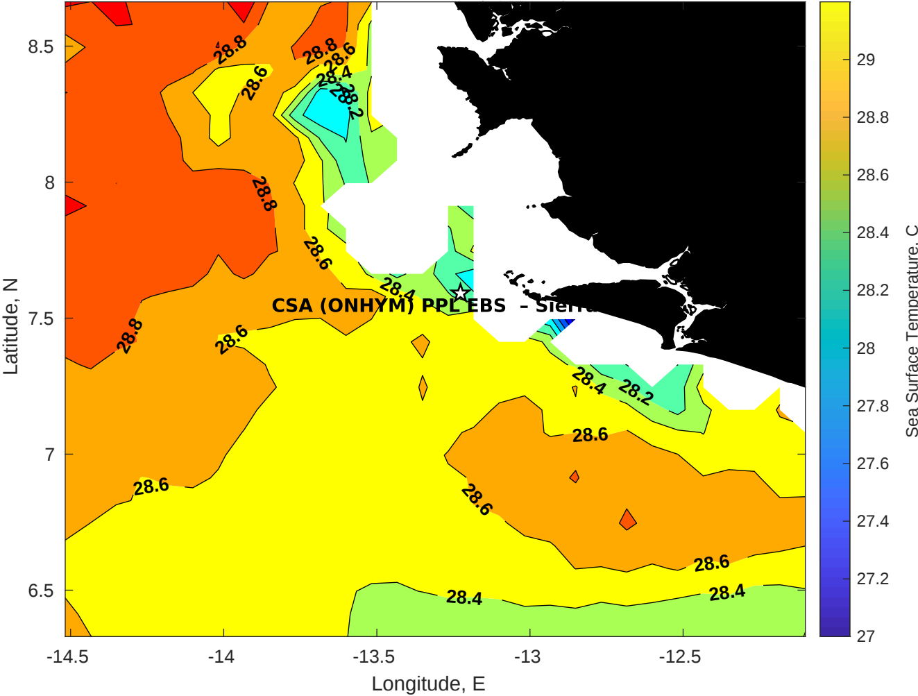
SST for CSA (ONHYM) PPL EBS - Sierra Leone at 25-Oct-2025 00:00:00
