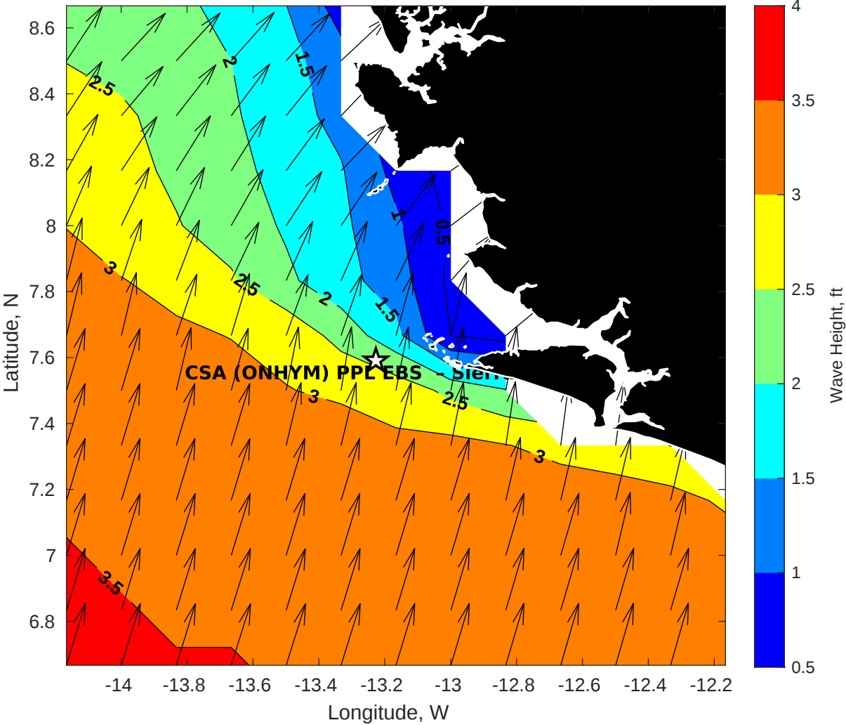
Wave Height (ft) for CSA (ONHYM) PPL EBS - Sierra Leone at 22-Oct-2025 21:00:00
