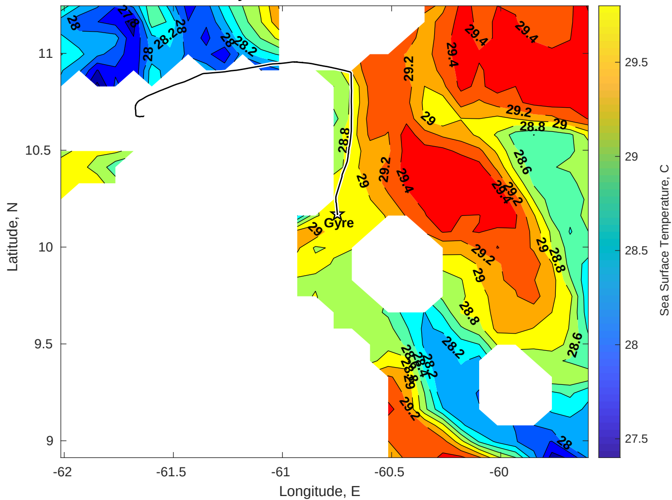
SST for Gyre at 25-Oct-2025 00:00:00
