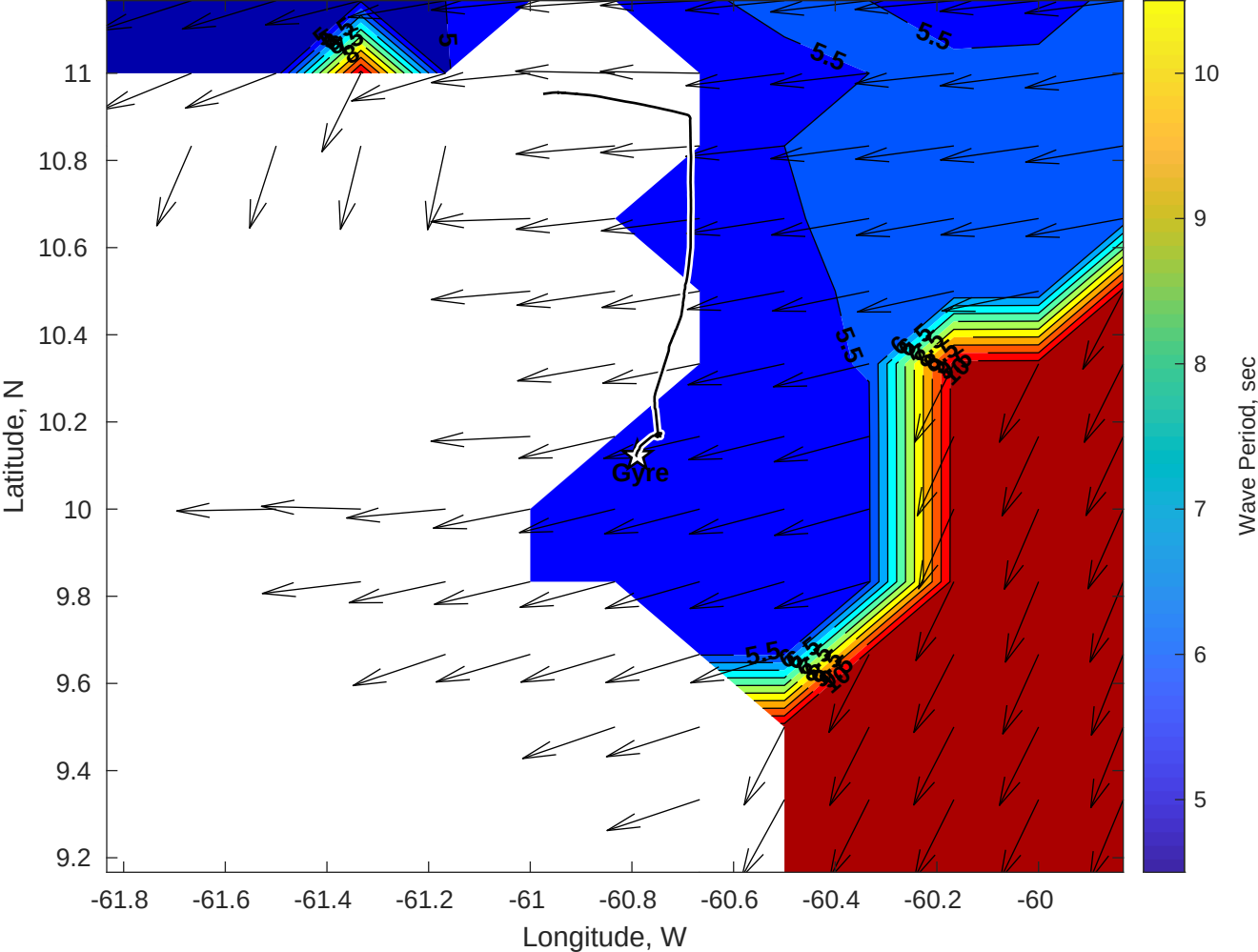
Wave Period (sec) for Gyre at 26-Oct-2025 09:00:00
