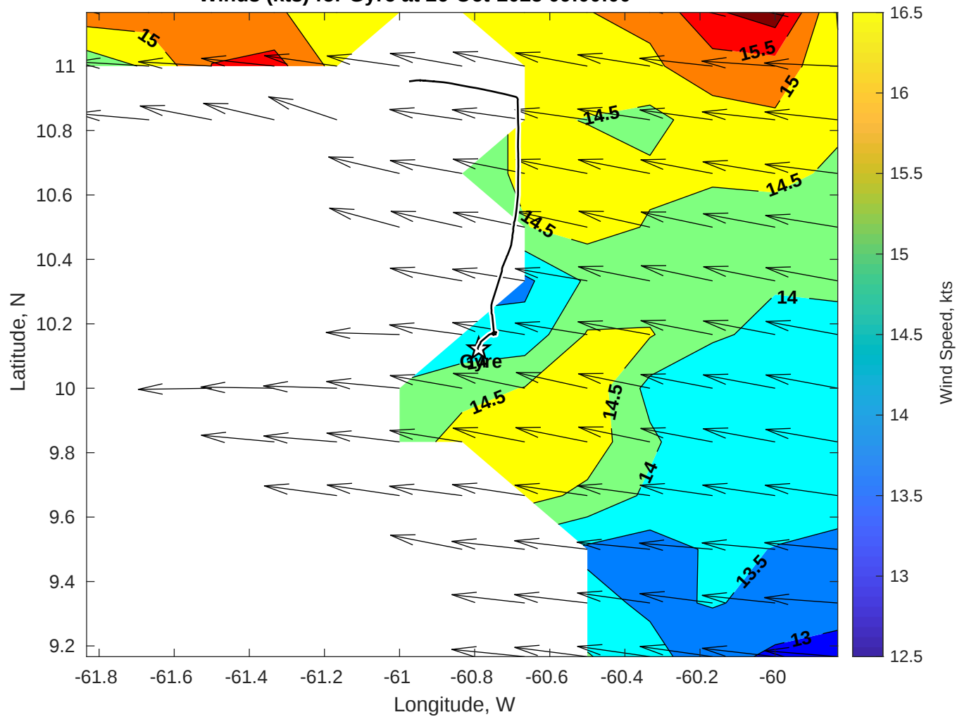
Winds (kts) for Gyre at 26-Oct-2025 09:00:00
