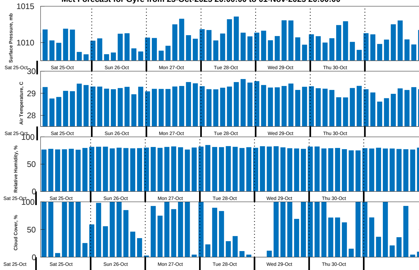
Met Forecast for Gyre from 25-Oct-2025 20:00:00 to 01-Nov-2025 20:00:00
