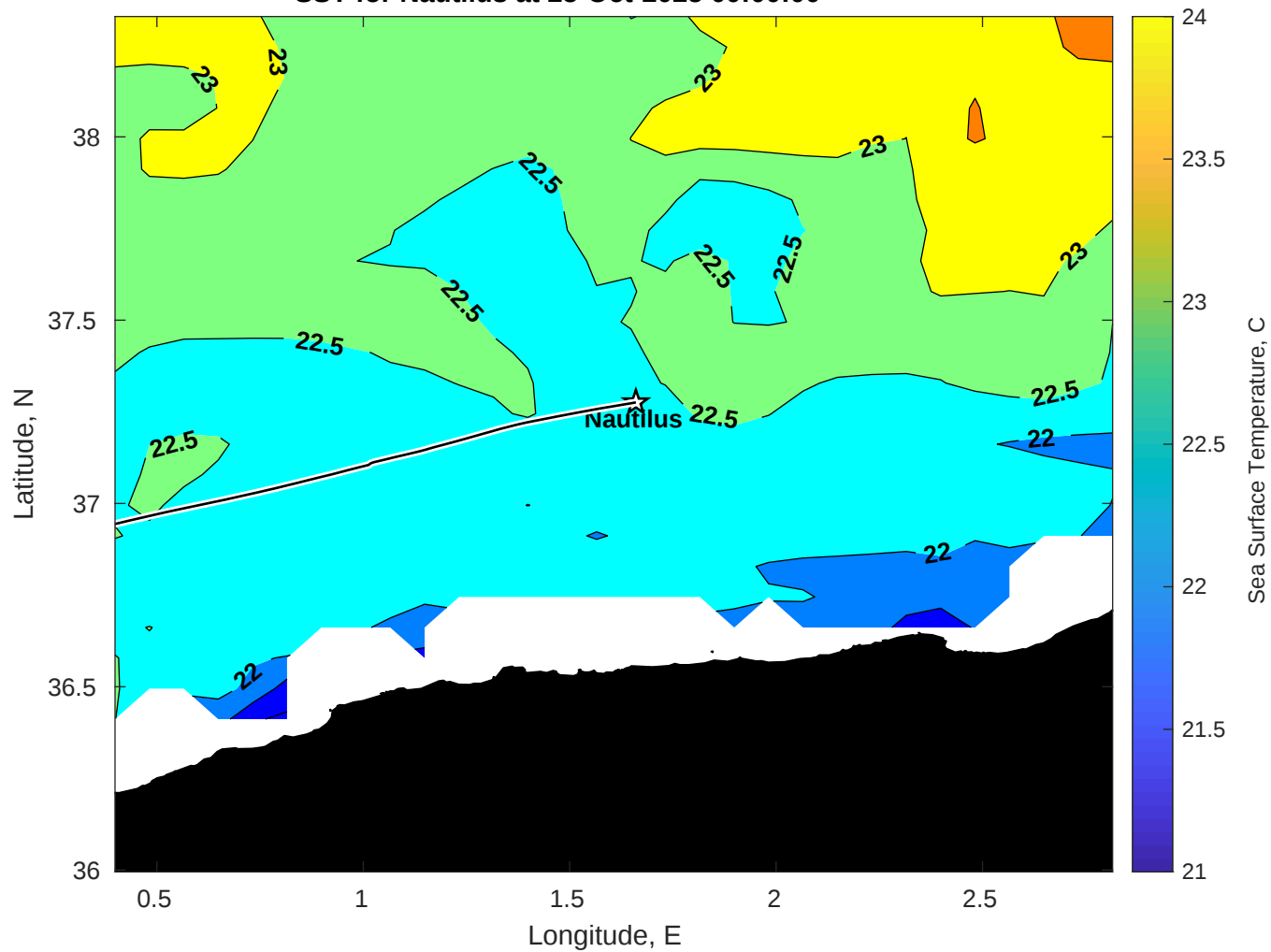
SST for Nautilus at 25-Oct-2025 00:00:00
