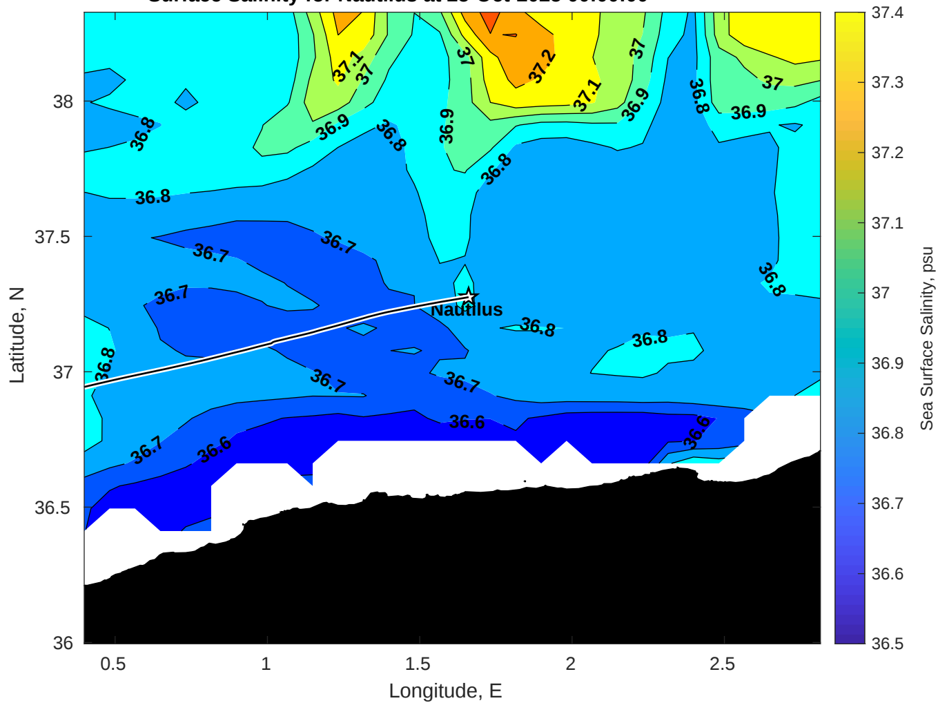
Surface Salinity for Nautilus at 25-Oct-2025 00:00:00
