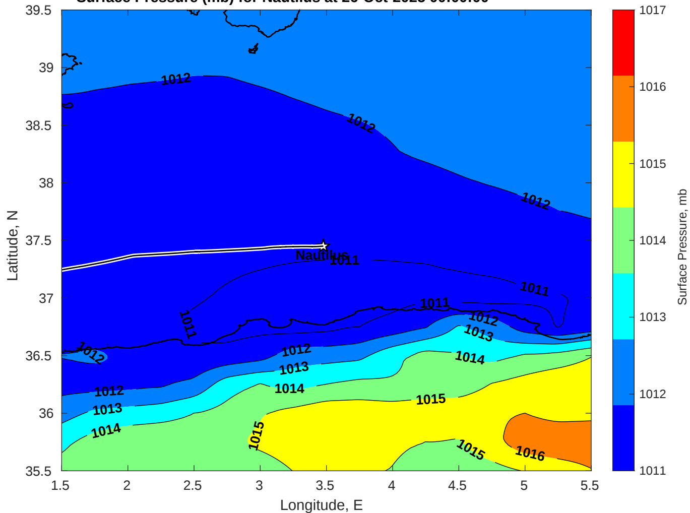
Surface Pressure (mb) for Nautilus at 26-Oct-2025 00:00:00
