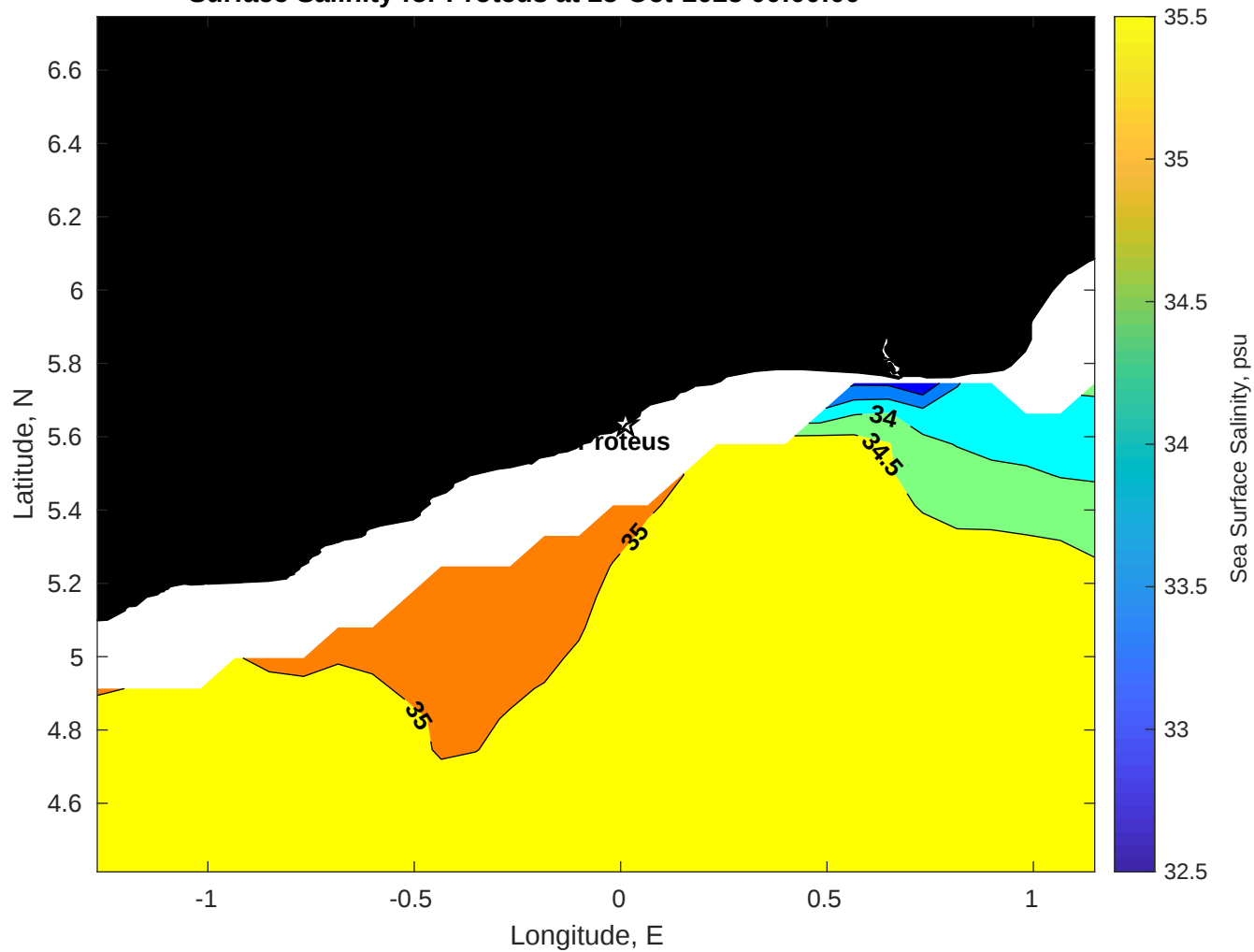
Surface Salinity for Proteus at 25-Oct-2025 00:00:00
